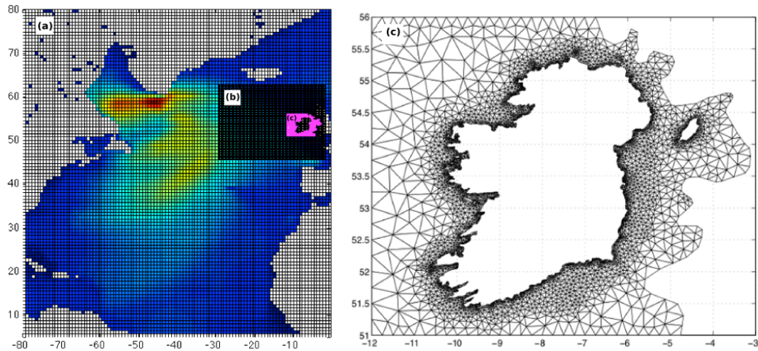
Figure 1. (a–c) The three wave model grids as described in Gallagher et al. (2016a). (a) The large North Atlantic grid has a 0.75^\circ \times 0.75^\circ resolution. (b) The grid for the Northeast Atlantic has a 0.25^\circ \times 0.25^\circ resolution. Right panel (c) The wave model unstructured grid around Ireland has a resolution ranging from 15 km offshore to 1 km in the nearshore characterised by 4473 nodes.
