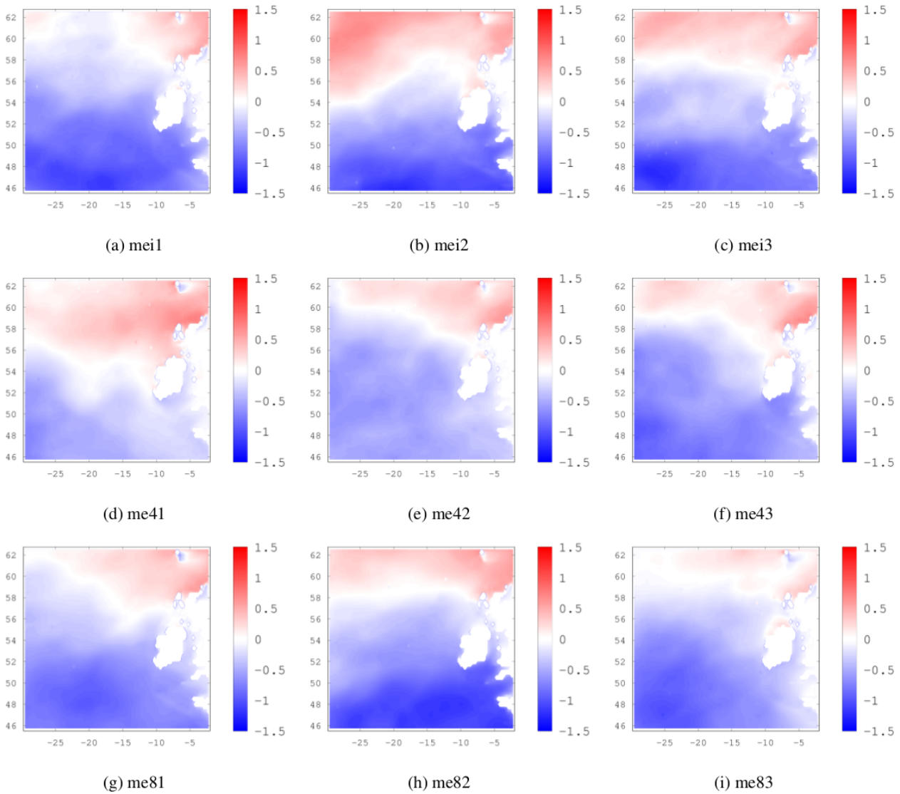
Figure B1. Maximum likelihood estimate of the \mu_2 parameter. The three ensemble members are shown for the historical period (a) to (c), future period under RCP4.5 (d) to (f), and future period under RCP8.5 (g) to (i).
