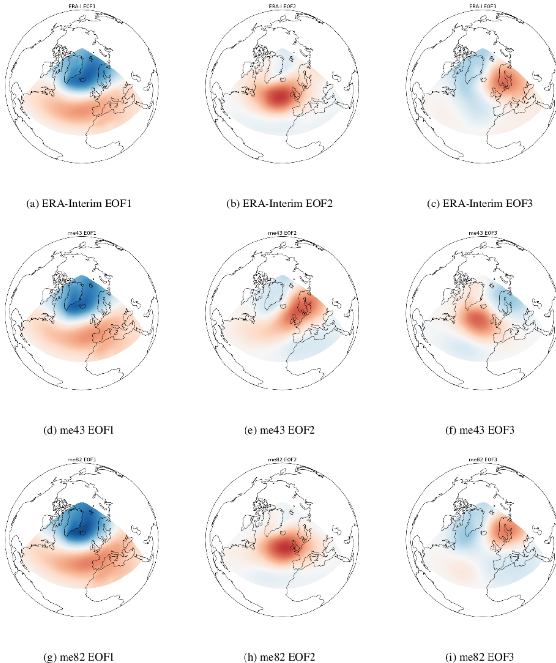
Figure 2. The first three EOF patterns for ERA-Interim (a) to (c), EC-Earth me43 (d) to (f) and EC-Earth me82 (g) to (i).
