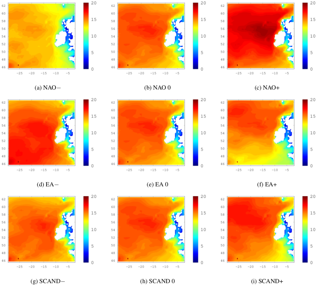
Figure 5. 20-year return levels of H_s where the effects of the NAO, EA and SCAND are isolated by setting each of the remaining two indices to zero. The ensemble mean is shown for the historical simulations.
