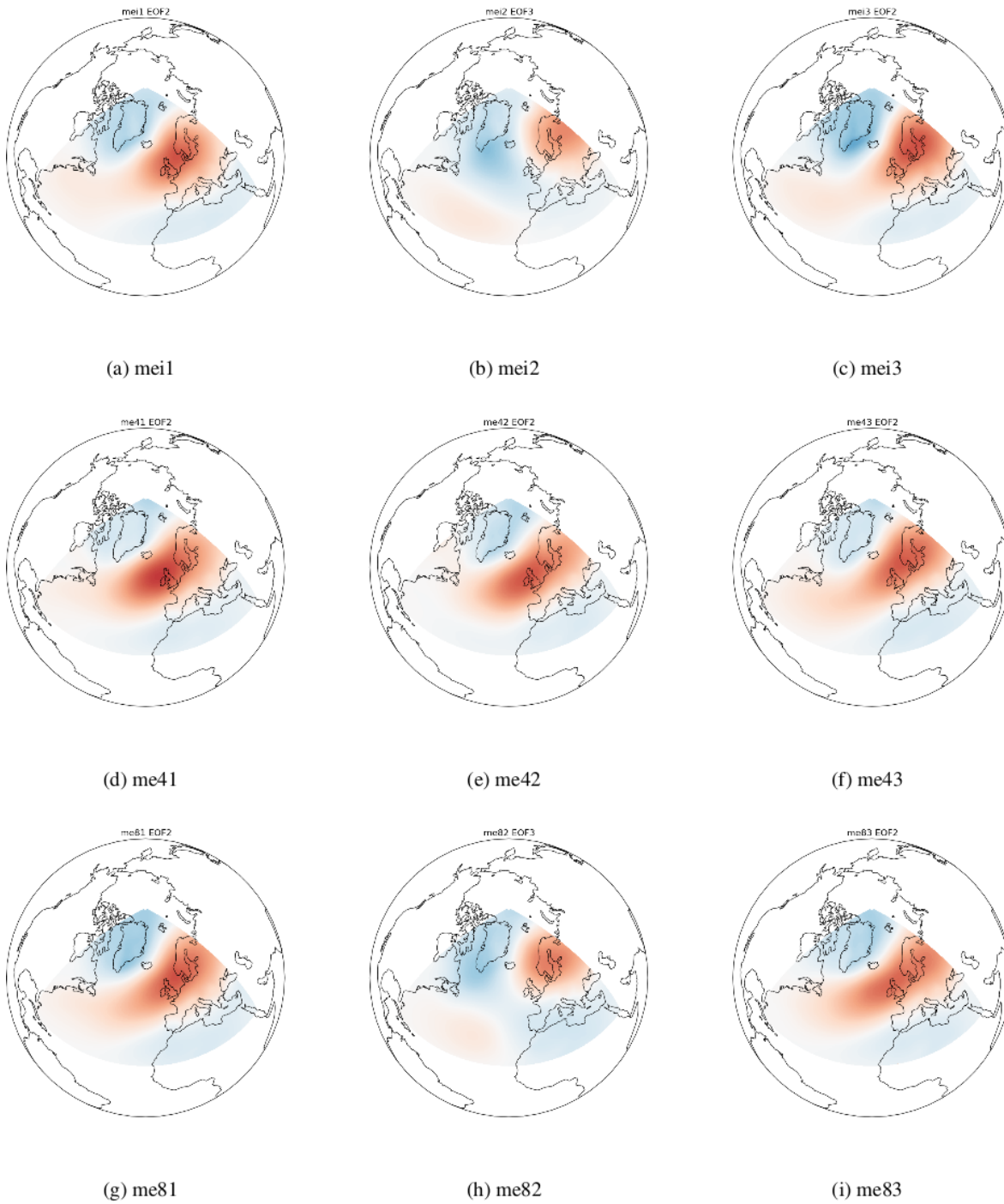
Figure A2. EOF patterns (2 or 3) corresponding to the SCAND teleconnection for the EC-Earth historical and future periods under RCP4.5 and RCP8.5.
