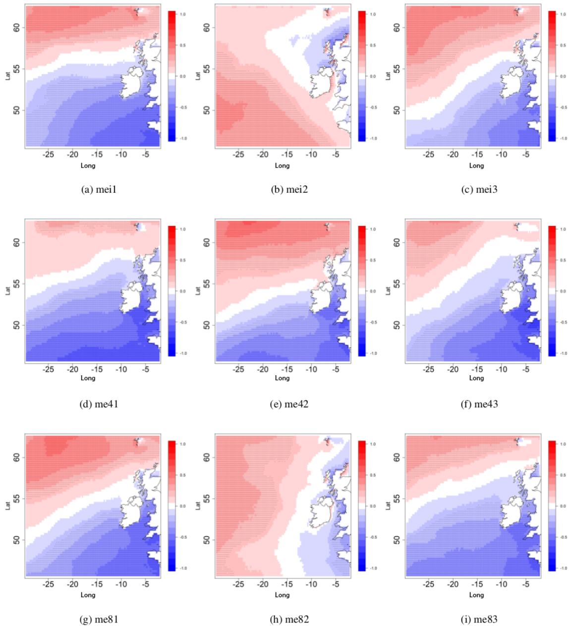
Figure 4. The Spearman correlation coefficient between the SCAND index and the 95th percentile of H_s for DJFM. (a–c) historical period (1980–2009) 3 \times ensemble members; (d–f) future period 2070–2099 under RCP4.5 and similarly (g–h) is for 2070–2099 under RCP8.5. Correlations statistically significant at the \alpha < 0.05 level are dotted.
