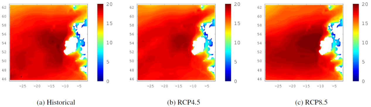
Figure 6. Ensemble mean 20-year return levels of H_s where the NAO is set to +2 and both the EA and SCAND are -2. A positive phase NAO and negative phase EA and SCAND is associated with the highest waves off Ireland.
