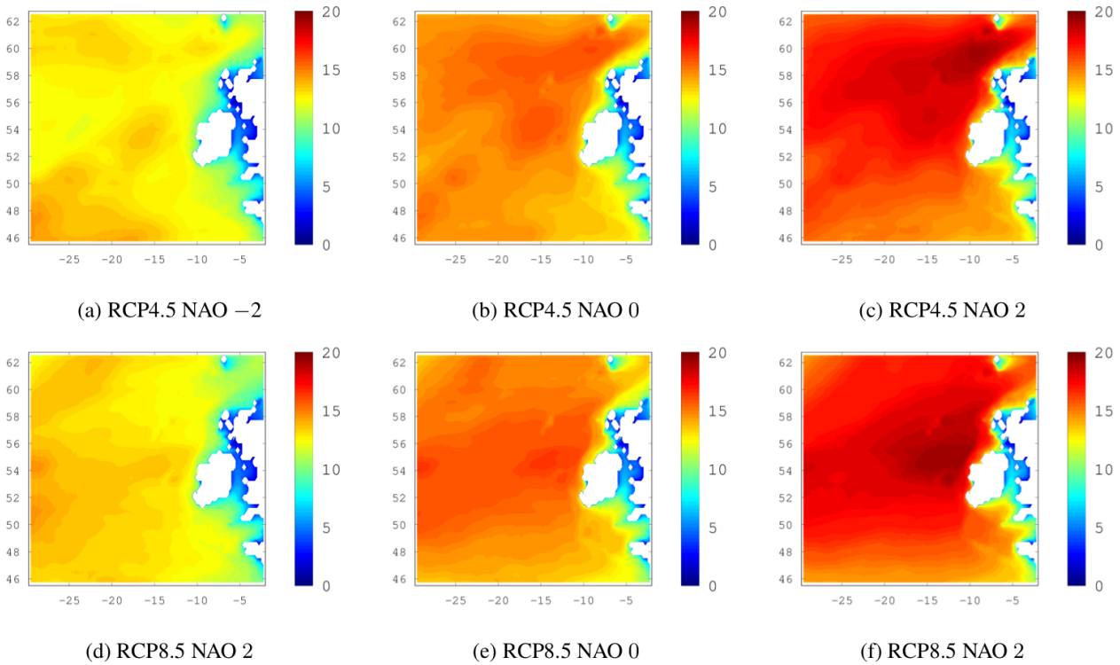
Figure C1. 20-year return levels of H_s . The NAO index varies from 3 values of the NAO index while the EA and SCAND are held in their neutral state (zero). The top row shows the ensemble mean for the future period under RCP4.5 and the bottom row is similar but shows RCP8.5 results.
