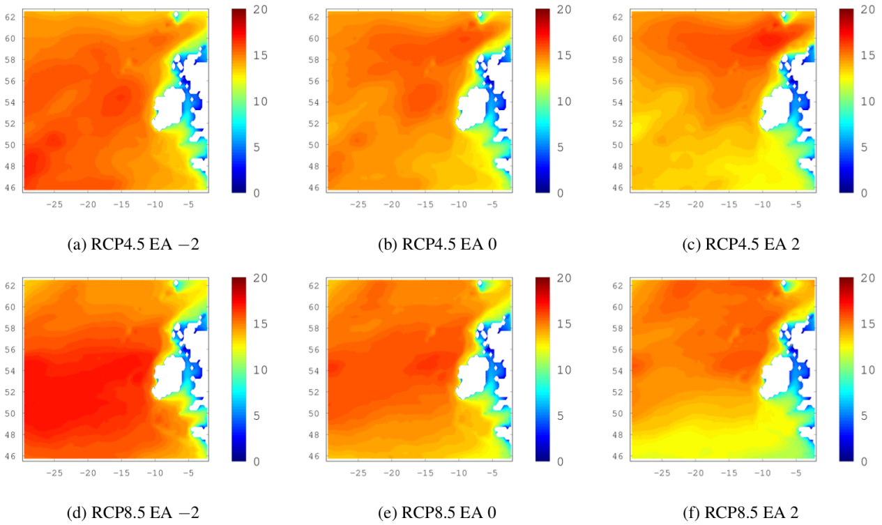
Figure C2. 20-year return levels of H_s . The EA index varies from 3 values of the NAO index while the NAO and SCAND are held in their neutral state (zero). The top row shows the ensemble mean for the future period under RCP4.5 and the bottom row is similar but shows RCP8.5 results.
