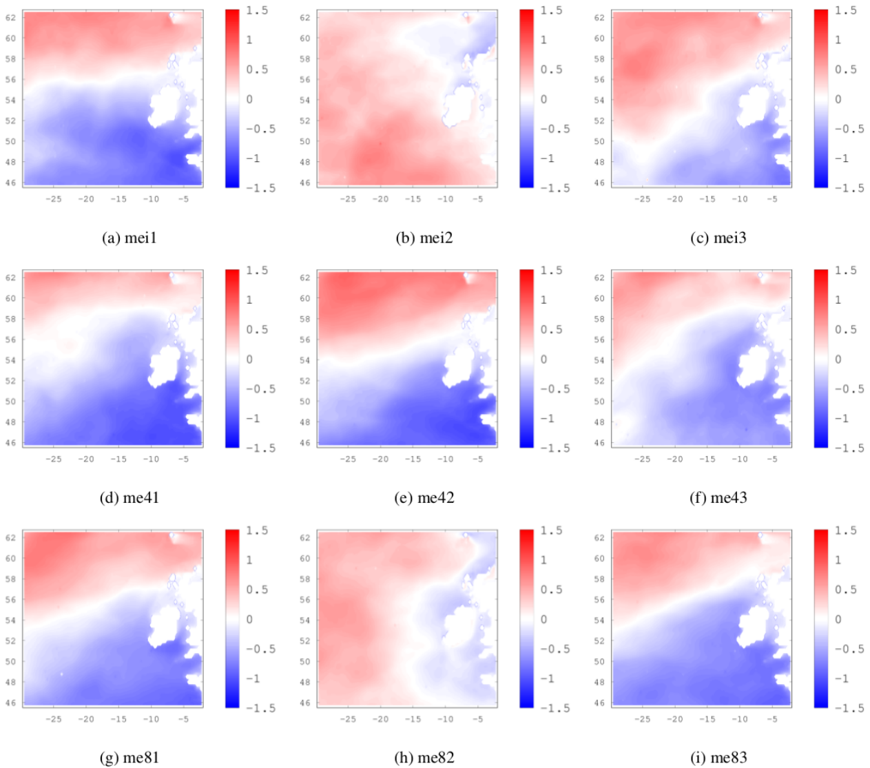
Figure B2. Maximum likelihood estimate of the \mu_3 parameter. The three ensemble members are shown for the historical period (a) to (c), future period under RCP4.5 (d) to (f), and future period under RCP8.5 (g) to (i).
