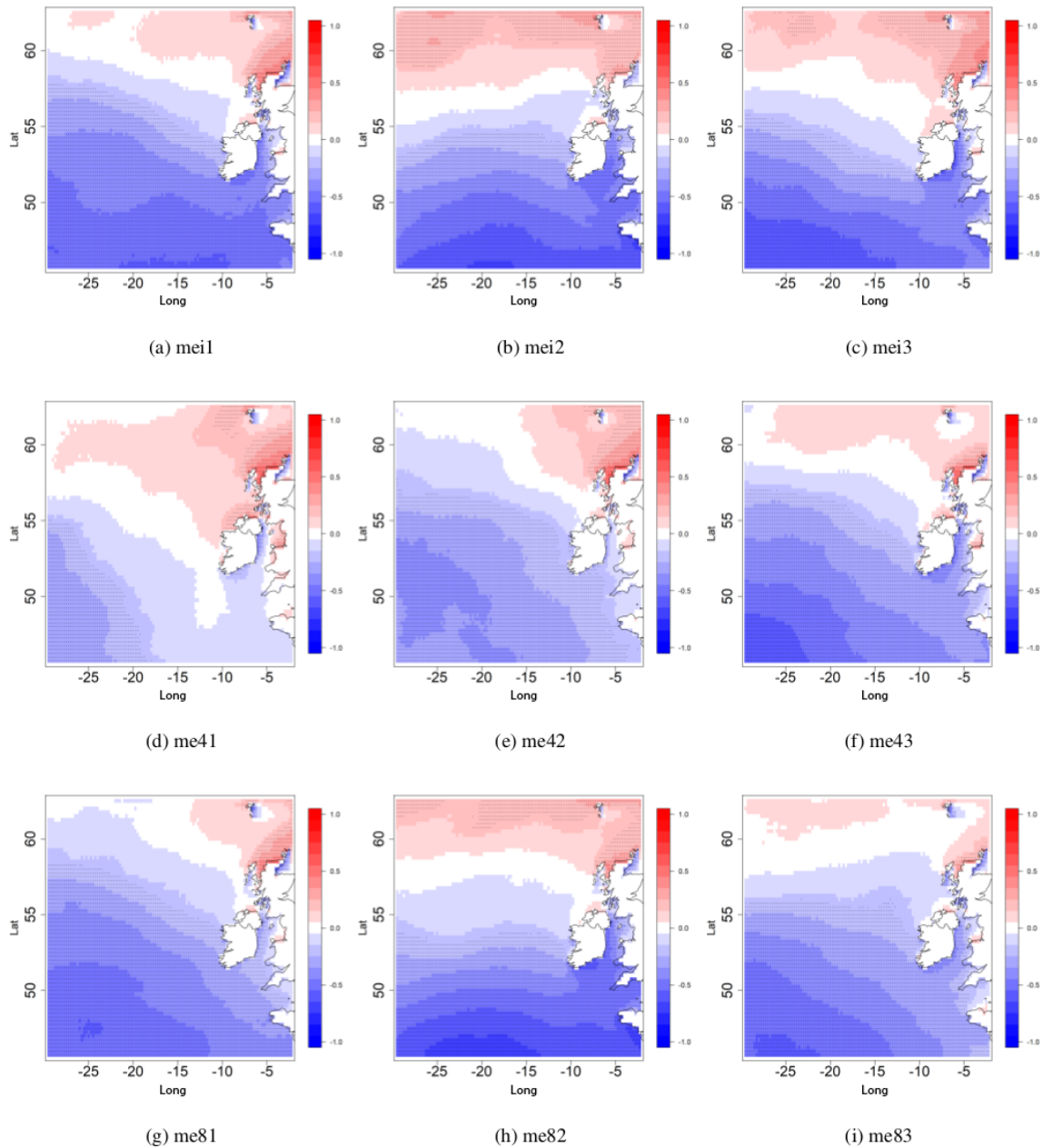
Figure 3. The Spearman correlation coefficient between the EA index and the 95th percentile of H_s for DJFM. (a–c) historical period (1980–2009) 3\times ensemble members; (d–f) future period 2070–2099 under RCP4.5 and similarly (g–h) is for 2070–2099 under RCP8.5. Correlations statistically significant at the \alpha < 0.05 level are dotted.
