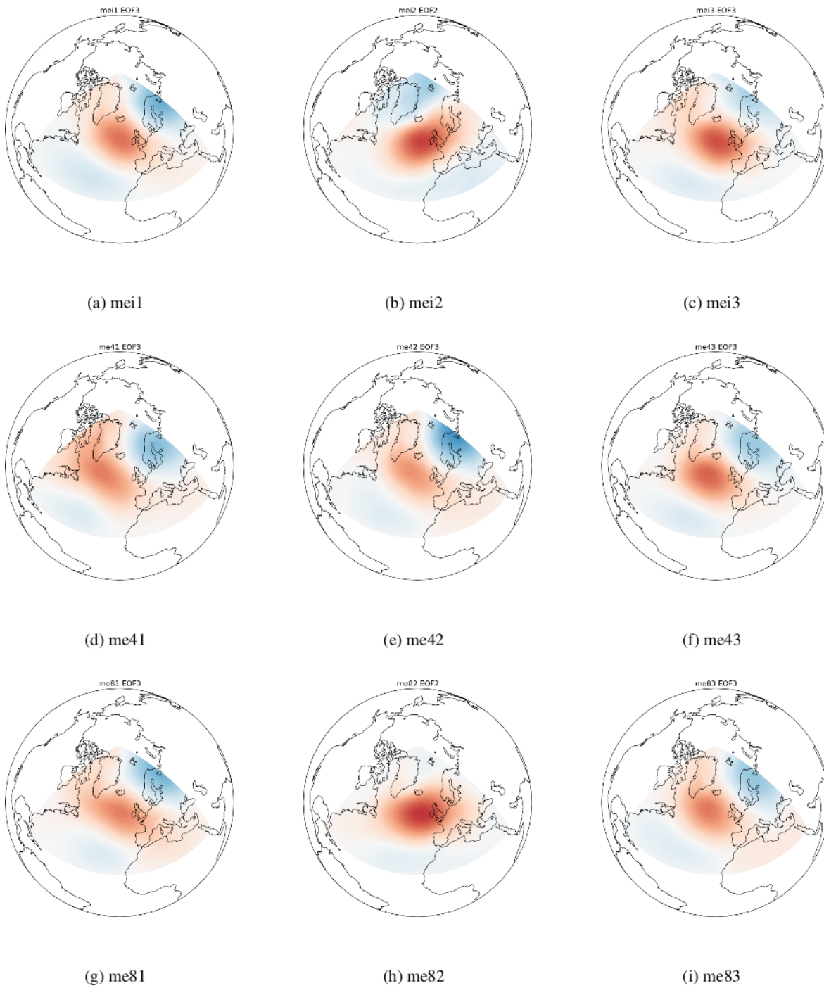
Figure A1. EOF patterns (2 or 3) corresponding to the EA teleconnection for the EC-Earth historical and future periods under RCP4.5 and RCP8.5.
