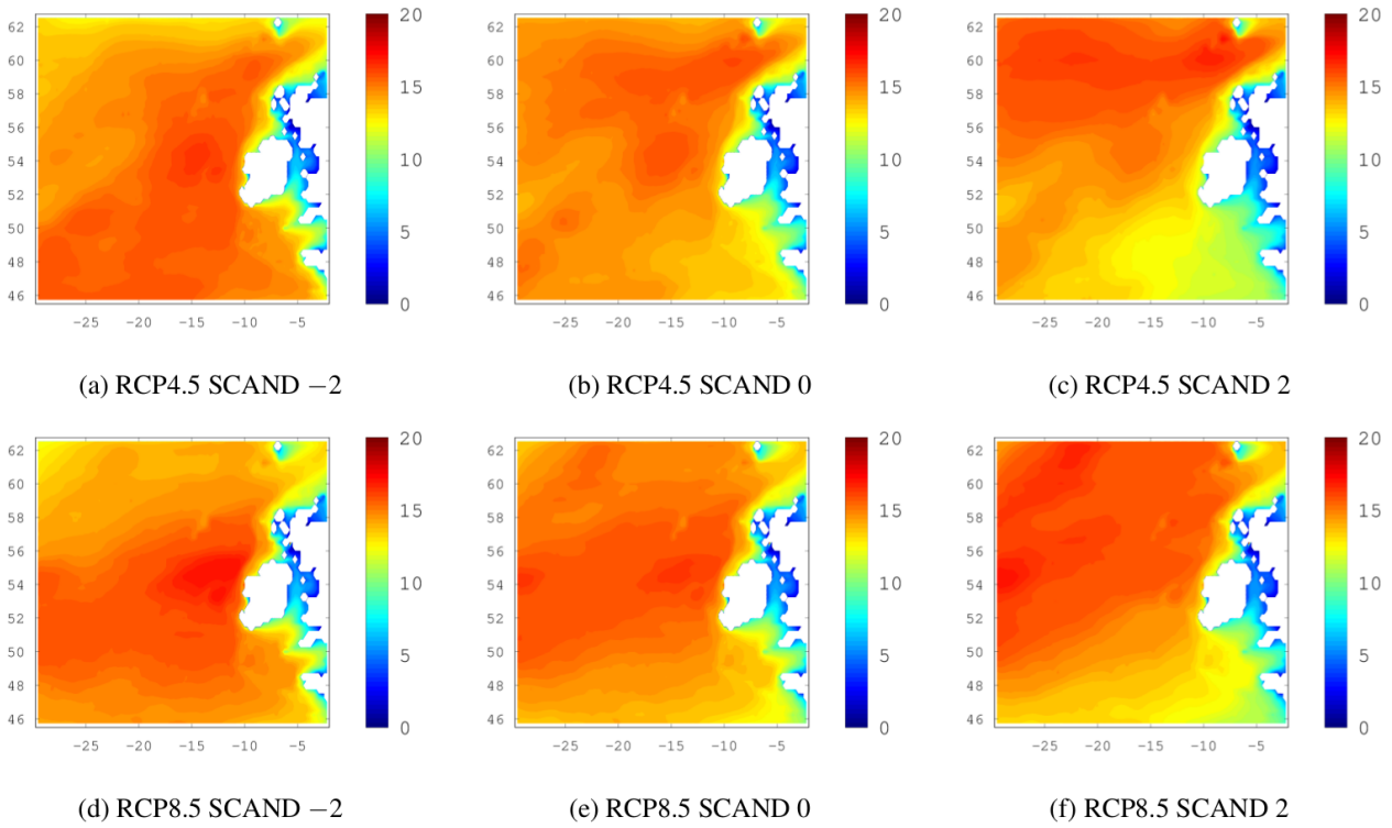
Figure C3. 20-year return levels of H_s . The SCAND index varies from 3 values of the NAO index while the NAO and EA are held in their neutral state (zero). The top row shows the ensemble mean for the future period under RCP4.5 and the bottom row is similar but shows RCP8.5 results.
