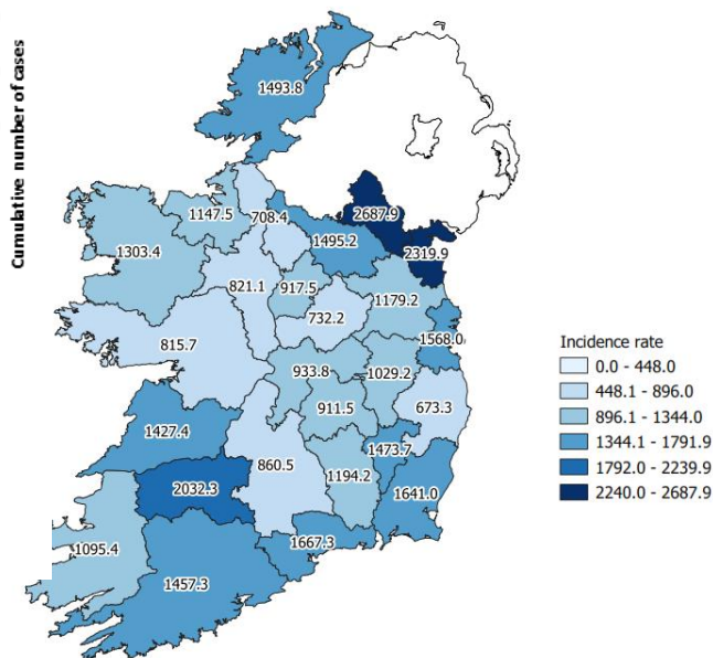
Cumulative incidence rates of confirmed cases of COVID-19 per 100,000 population notified in Ireland between 28/12/2020 and 10/01/2021
