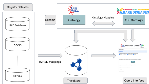
Fig. 1. Relation between FAIRVASC and CDE ontologies
