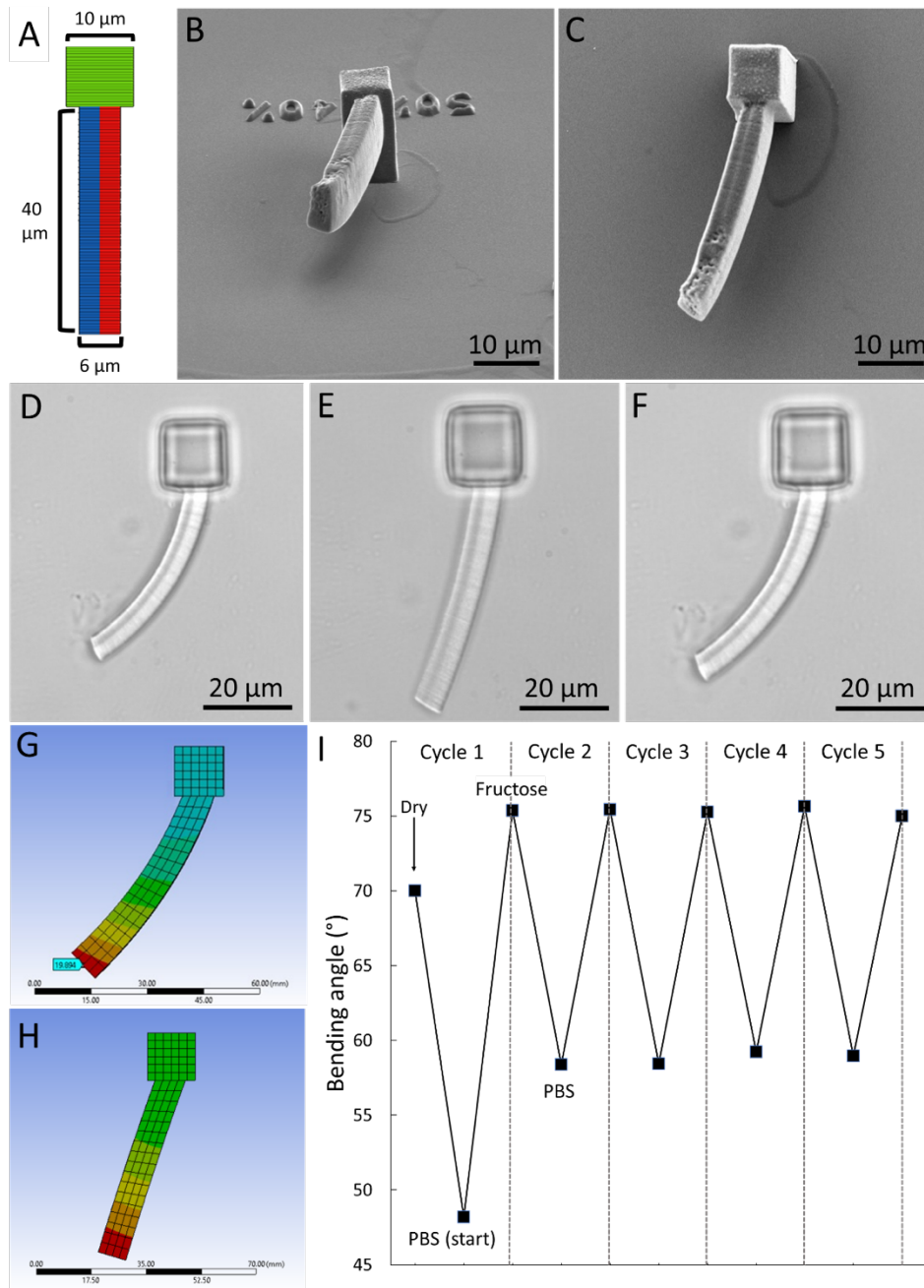
Figure 5. Responsive bilayer beams. (A) Design of the bilayer beam, red denotes volume fabricated at 25 mW laser power, blue denotes volume fabricated 20 mW laser power and green denotes the base of the beam fabricated at 30 mW; (B) SEM image of beam structure at 60 °; (C) Top down SEM image of beam structure; Optical microscope image of (D) beam bending while hydrated in PBS; (E) Beam straightening while in 5 mM fructose solution; (F) beam bending when the hydration media is reverted to PBS; FEA models of beam in (G) PBS solution and (H) 5 mM fructose; (I) graph showing the bending angle of the beam through multiple PBS to 5 mM fructose cycles.
