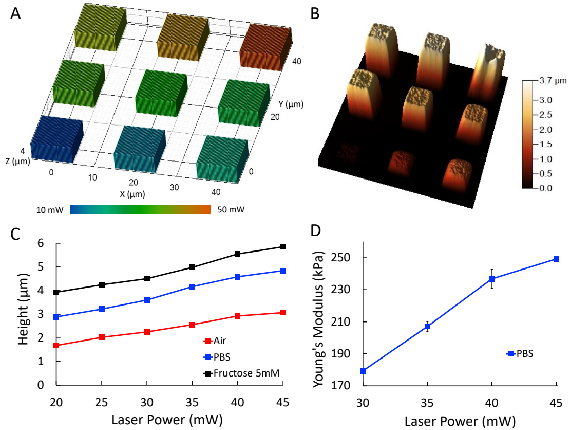
Figure 3. Height profiles and Young's modulus measurements of the micro-cubes. (A) Design of the array of 10 \mu\text{m} \times 10 \mu\text{m} \times 4 \mu\text{m} cubes fabricated at different laser powers (10 to 50 mW) used for all AFM measurements; (B) 3D height plot of the micro-cube array fabricated at 10 to 50 mW in the dry state; (C) Graph showing height of cubes at each laser power, in the dry state, PBS, and fructose 5mM. (D) Graph showing Young's modulus of micro-cubes fabricated at different laser power upon hydration in PBS.
