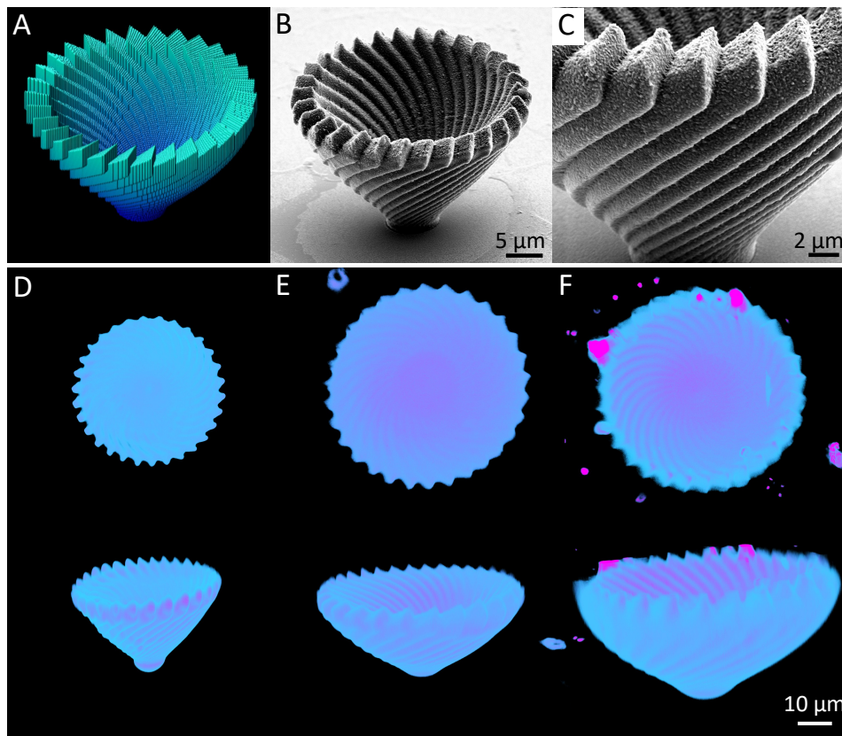
Figure 4. Complex 3D soft hydrogel vase structure. (A) Design of twisted vase structure of 23 \mu\text{m} in height, with a top diameter of 32 \mu\text{m} and a base diameter of 6.6 \mu\text{m} ; (B) SEM image and (C) SEM detail of the vase structure fabricated at a laser power of 25 mW and 10 mm \text{s}^{-1} . (D, E, F) confocal microscopy images showing top-down view and side profile of the 3D vase in the dry state, hydrated in PBS and in 100 mM fructose solution, respectively.
