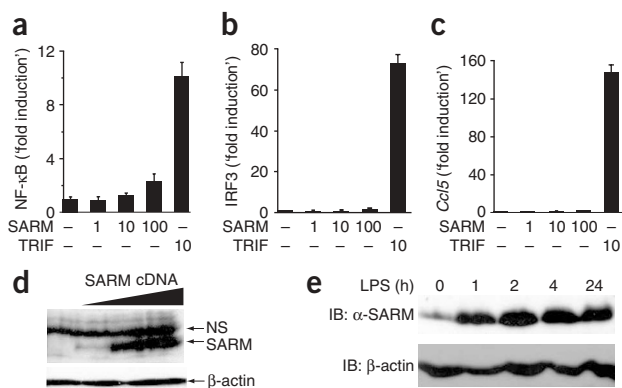
Figure 1 Expression of SARM fails to activate NF-κB or IRF3.
