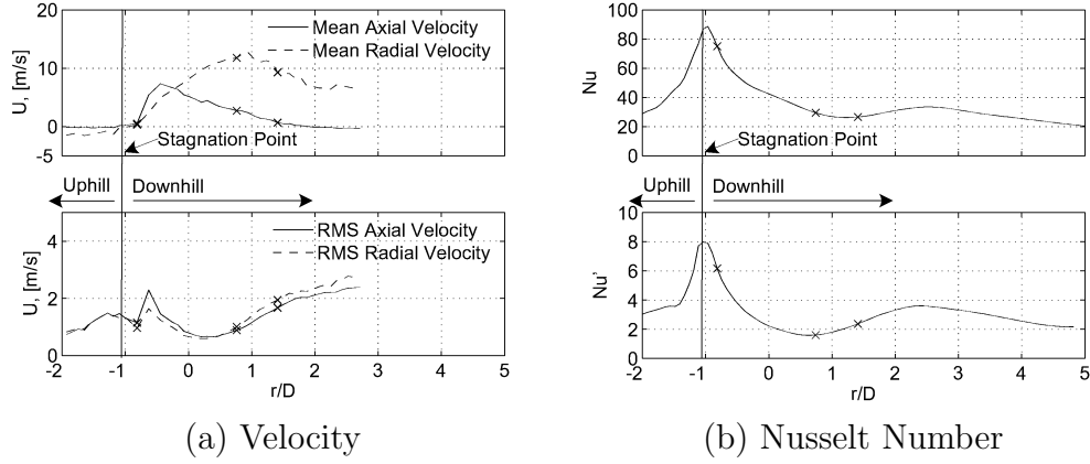
Fig. 7. Velocity & Heat Transfer Distributions; H/D = 2 ; \alpha = 45^\circ
