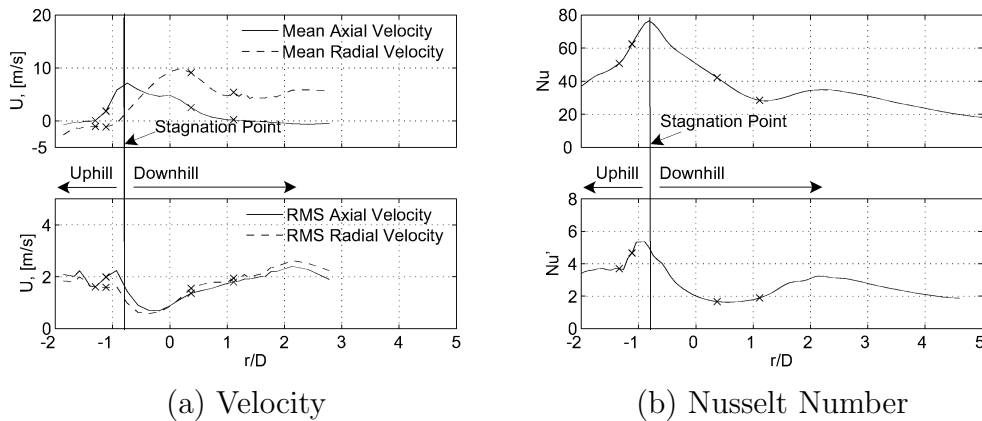
Fig. 12. Velocity & Heat Transfer Distributions; H/D = 2 ; \alpha = 60^\circ
