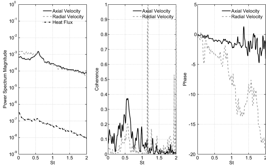
Fig. 10. Power spectra and coherence and phase information between velocity and heat flux signals; H/D = 2 , \alpha = 45^\circ , r/D = 0.8
