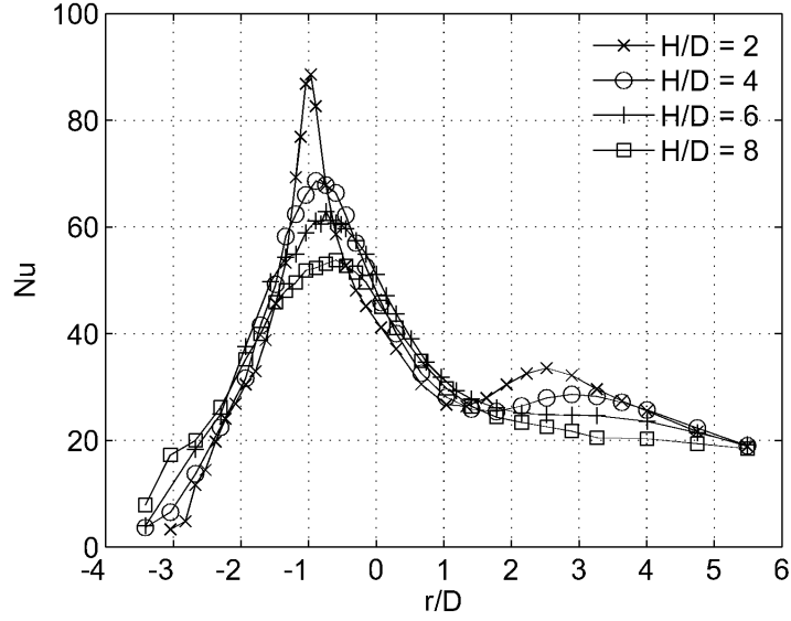
(a) Mean Nu
