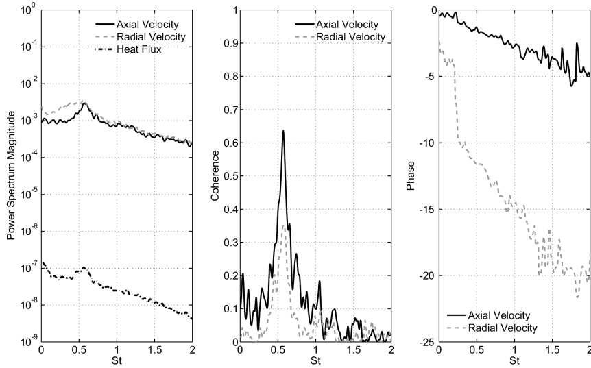
Fig. 15. Power spectra and coherence and phase information between velocity and heat flux signals; H/D = 2 , \alpha = 60^\circ , r/D = 0.4
