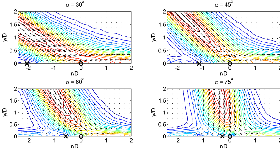
Fig. 2. Velocity Flow Fields for an Obliquely Impinging Jet, H/D = 6
