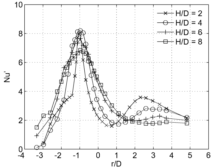
(b) Root-Mean-Square Nu'
