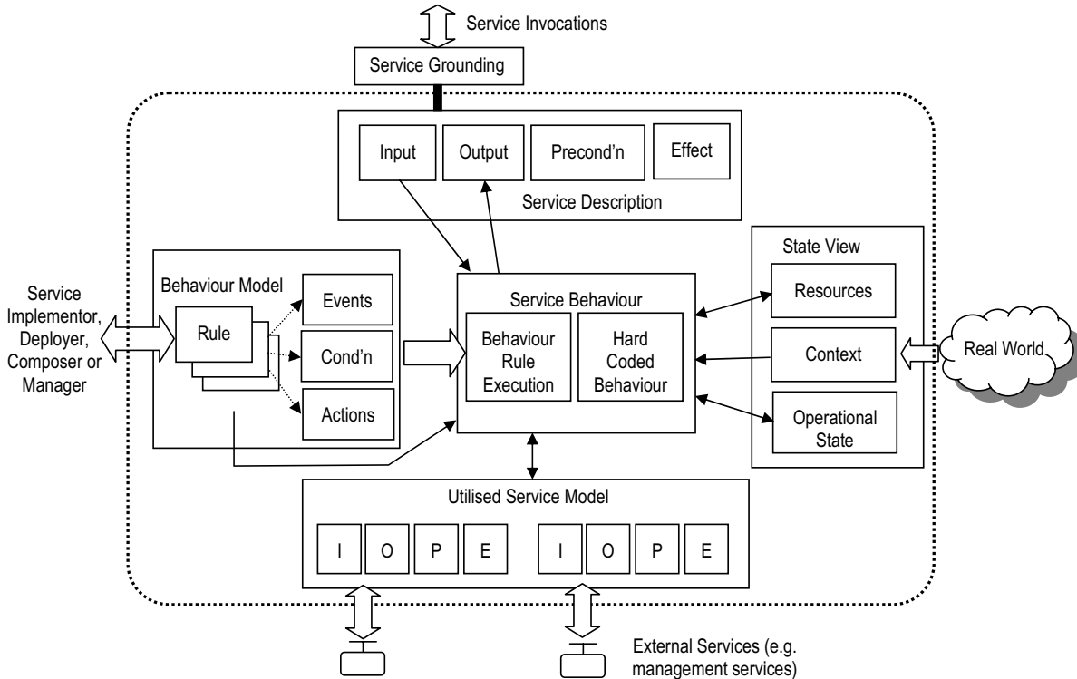
Figure 3: Anatomy of an Adaptive Service Element
