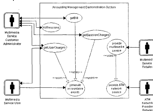
Figure 5: Accounting Trial - Use Case Summary
