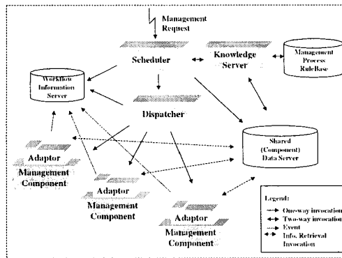
Figure 4 TMWE Architecture
