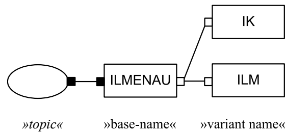
Fig. 2. Base name and variant names
