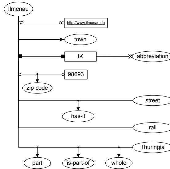
Fig. 11. Subject centric view of GTM alpha
