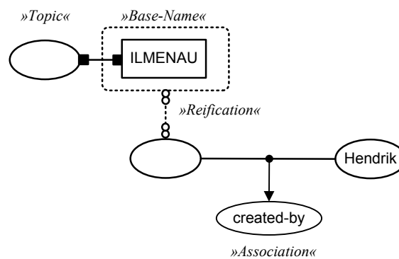
Fig. 9. Reification
