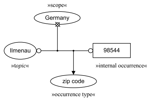
Fig. 7. Occurrence with type and scope
