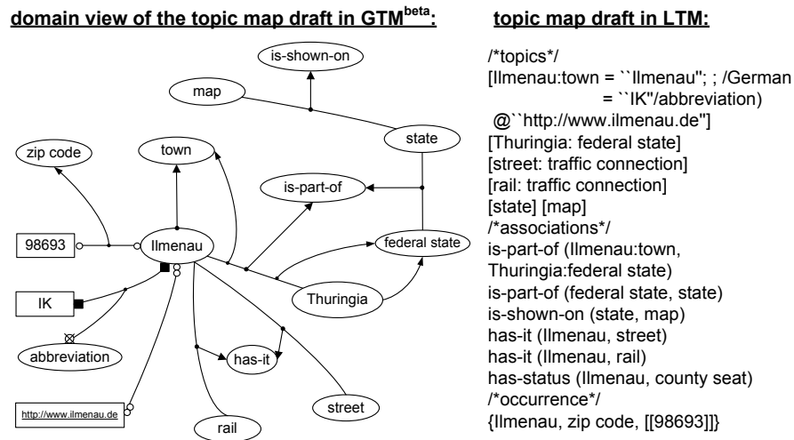
Fig. 10. Domain view of GTM alpha
