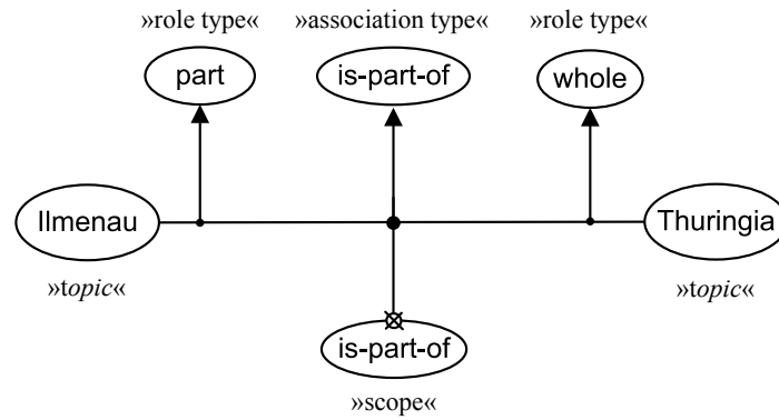
Fig. 8. Association
