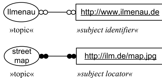
Fig. 5. Subject locator and subject identifier
