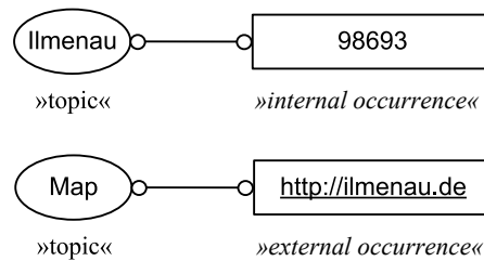
Fig. 6. Internal and external occurrence
