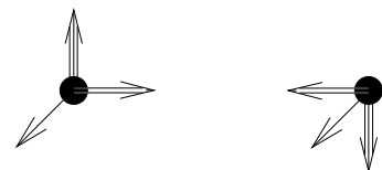
Figure 1: Two Skyrmions attracting. The different arrow types correspond to different dipoles.
