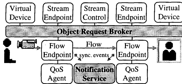
Figure 3. The Quartz/CORBA framework
