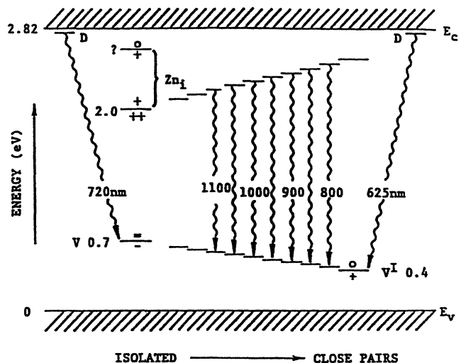
FIG. 3. Schematic diagram showing the energy-level positions and optical transitions for the isolated zinc vacancy, the isolated zinc interstitial, and the zinc Frenkel pairs.
