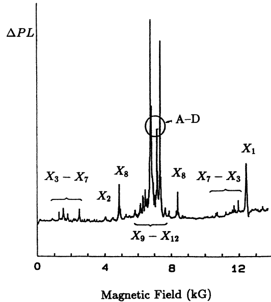
FIG. 1. ODMR spectrum detected from the total near-infrared luminescence in e^- -irradiated ZnSe at 1.5 K with B \parallel [111] and \nu = 20 GHz.
