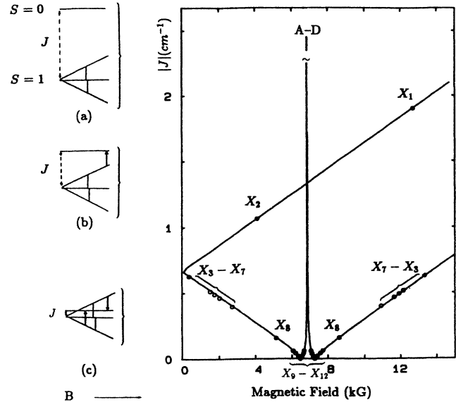
FIG. 2. Predicted magnetic field positions (solid lines) for the transitions of two exchange coupled particles vs |J| for g_I = 1.9664 , (g_V)_\perp = 2.2085 , \nu = 20 GHz, and \bar{D}_i = 0 in Eq. (1). The circled points are the experimental points for the indicated spectra. The insets (a)-(c) illustrate the schematic energy level schemes as a function of J .
