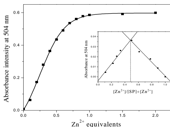
Figure 6. Absorption intensities at 504 nm of a solution of spiropyran SP ( 1.0 \times 10^{-4} M, \text{CH}_3\text{CN} , 293K) after increasing the concentration of \text{Zn}(\text{ClO}_4)_2 ; (Inset) Job's analysis of ME-Zn complex ( [\text{SP}] + [\text{Zn}^{2+}] = 3.0 \times 10^{-5} M, \text{CH}_3\text{CN} , 293K).
