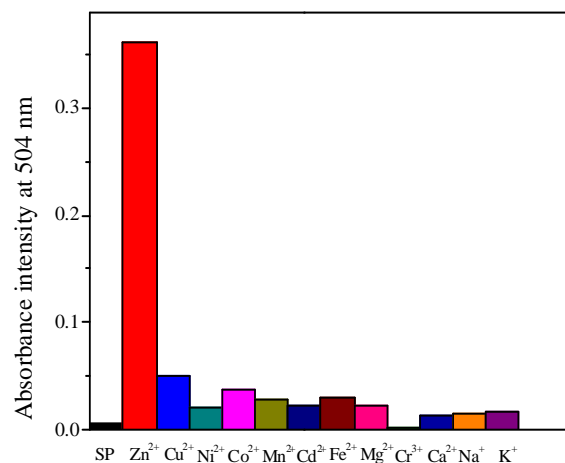
Figure 3. Absorption intensity at 504 nm of solutions of spiropyran SP ( 1.0 \times 10^{-4} M, \text{CH}_3\text{CN} , 293K) before and after the addition of 1 equivalent of \text{Zn}(\text{ClO}_4)_2 , \text{Cu}(\text{ClO}_4)_2 , \text{Ni}(\text{ClO}_4)_2 , \text{Co}(\text{ClO}_4)_2 , \text{Mn}(\text{ClO}_4)_2 , \text{Cd}(\text{ClO}_4)_2 , \text{Fe}(\text{ClO}_4)_2 , \text{Mg}(\text{ClO}_4)_2 , \text{Cr}(\text{ClO}_4)_3 , \text{CaCl}_2 , \text{NaCl} and \text{KCl} .
