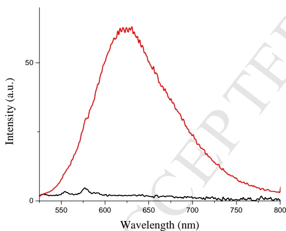
Figure 5. Emission spectra of a solution of ( 1.0 \times 10^{-5} M, \text{CH}_3\text{CN} , 293K, \lambda_{\text{exc}} = 492 nm) before (black) and after the addition of 1 equivalent of \text{Zn}(\text{ClO}_4)_2 (red).
