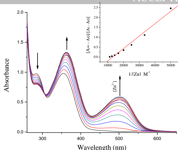
Figure 7. (a) The absorption spectra of a solution of SP ( 1.0 \times 10^{-4} M, \text{CH}_3\text{CN} , 293K) after 20 minutes from the addition of 0.1, 0.2, 0.3, 0.4, 0.5, 0.6, 0.7, 0.8, 0.9, 1, 1.5, 2 equivalent of (\text{Zn}(\text{ClO}_4)_2) ; (Inset) Plot of (A_\infty - A_0)/(A_x - A_0) against 1/[\text{Zn}] , binding constant k = 1.6 \times 10^4 \text{ M}^{-1} .
