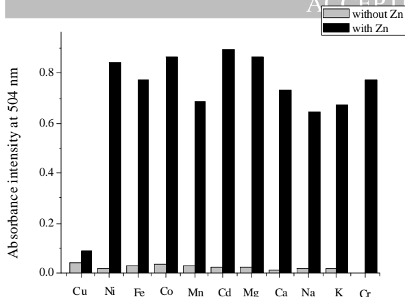
Figure 4. Absorbance intensity responses of SP ( 1 \times 10^{-4} M in acetonitrile) to various metal ion. Grey bars represent the absorption of SP at 504 nm in the presence of 1 equivalent of a selected metal ion. Black bars represent the absorption of SP at 504 nm in the presence of a binary mixture of Zn(II) and a competitive metal ion (1 equivalent each).
