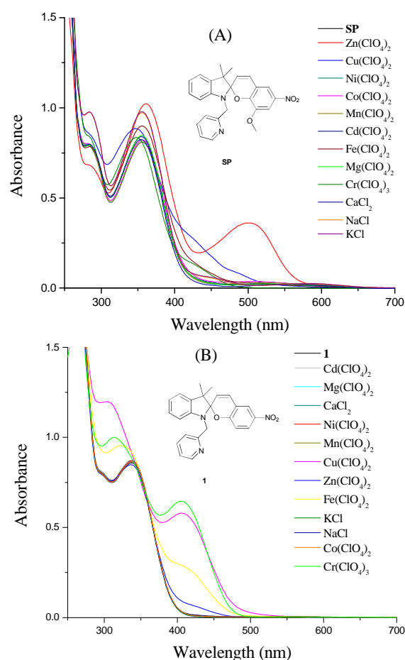
Figure 2. Absorption spectra of spiropyran SP ( 1.0 \times 10^{-4} M, \text{CH}_3\text{CN} , 293K) (A) and spiropyran 1 ( 1.0 \times 10^{-4} M, \text{CH}_3\text{CN} , 293K) (B) after 20 minutes from the addition of 1 equivalent of different metal perchlorates and chlorides.
