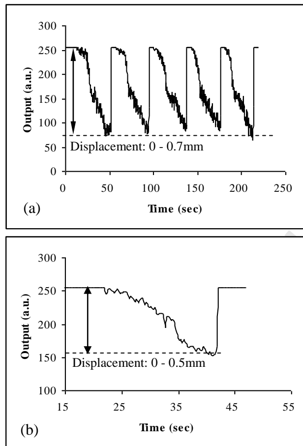
Fig. 9. Real-time response trace during a repeated compression test using Zwick instrument. Speed: 1 mm/min, maximum loading: 200N. (a) Pressing head at the center of the cover. (b) Pressing head 4mm away from the center of the cover.
