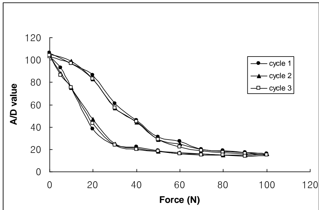
Fig. 10. Cyclic loading and unloading of the pressure sensing bite guard.
