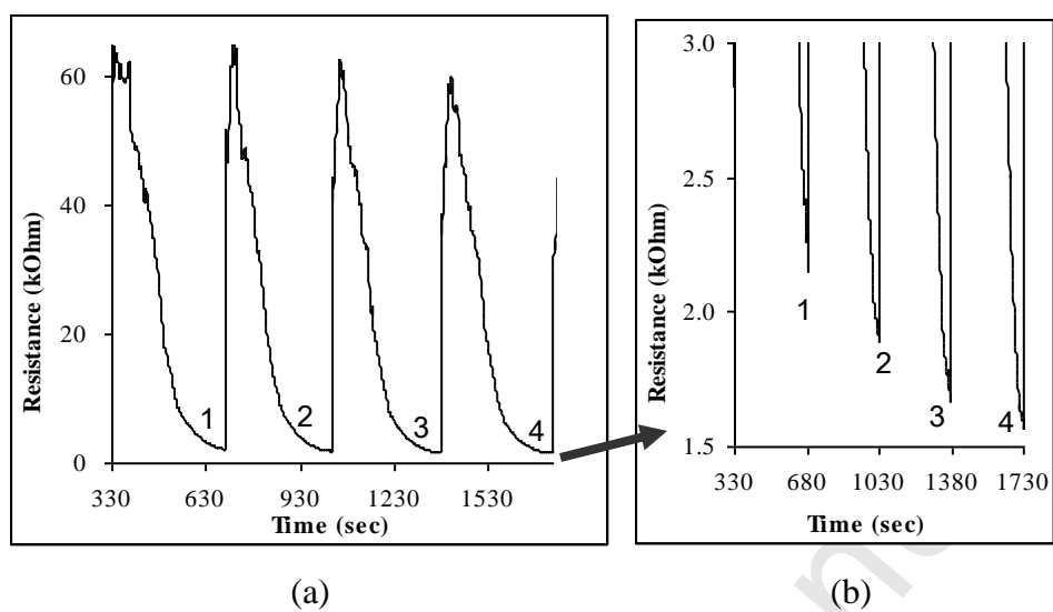
Fig. 5. Compressive test showing the repeatability of the pressure sensor. (Test speed: 0.1mm/min)
