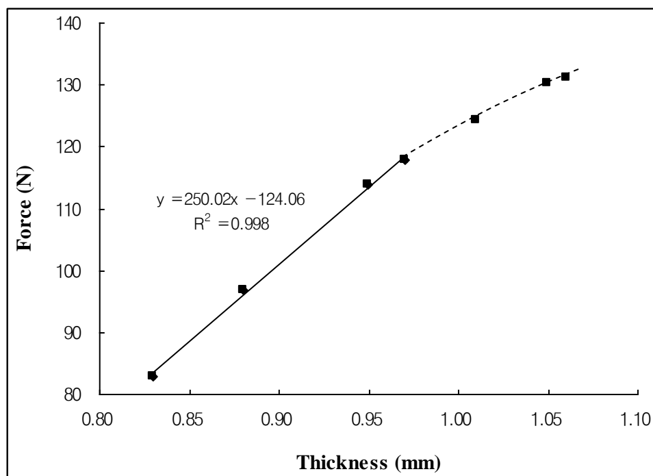
Fig. 6. Force-thickness curve with different thicknesses of acrylic cover.
