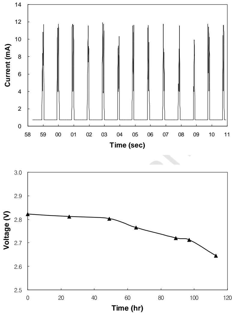
Fig. 8. (a) The current draw of microcontroller in transmitter module: Transmitting frequency = 1Hz (b) Voltage drop of battery during operation.
