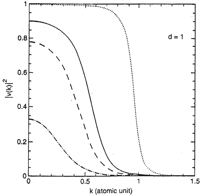
Figure 1. Occupancy v(k)^2 of the variational wavefunction at low and high densities. Note how it evolves from nearly a Fermi function at small r_s to a Lorentzian form (expected for a hydrogenic exciton) at low density. Dotted line: r_s = 2.11 ; thick solid line: r_s = 3.69 ; dashed line: r_s = 4.72 ; dotted-dashed line: r_s = 9.56 . The calculations are for coupled quantum wells at a separation of 1 Bohr radius. From [40].
