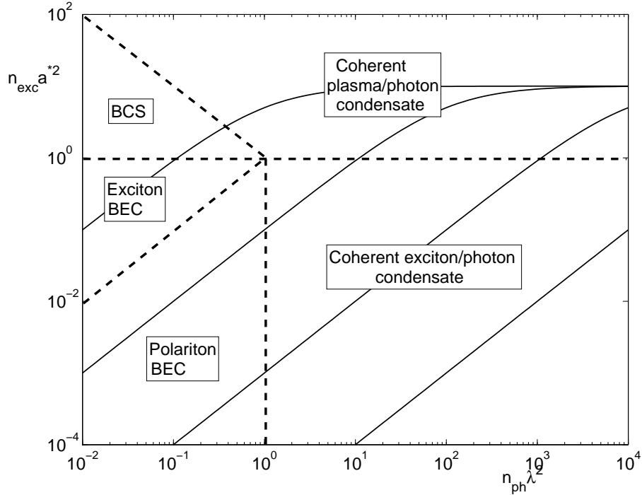
Figure 6. Sketch to demonstrate the various crossovers in the polariton problem. The dimensionless densities are plotted on the two axes n_{exc}a^{*2} for excitons and n_{ph}\lambda^2 = n_{ph}\hbar^2/2M^*g for photons. The crossover from BEC of polaritons to an interaction-driven polariton condensate occurs when n_{ph}\lambda^2 \approx 1 ; the conventional BEC/BCS crossover for excitons occurs when n_{exc}a^{*2} \approx 1 , and at large photon numbers this marks the conventional point of inversion for a plasma “laser”. The two wedges labelled BCS and exciton BEC constitute the regime where the Coulomb interaction is the dominant coupling term. The solid lines are rough guides to trajectories that would be followed for a fixed ratio of the coupling constants (a^*/\lambda)^2 = (g/Ryd.)(M^*/m) = 10, 10^{-1}, 10^{-3}, 10^{-5} . In order for the electron-hole density to be able to reach such high values as shown, the cavity mode frequency would need to be placed well above the edge of the band.
