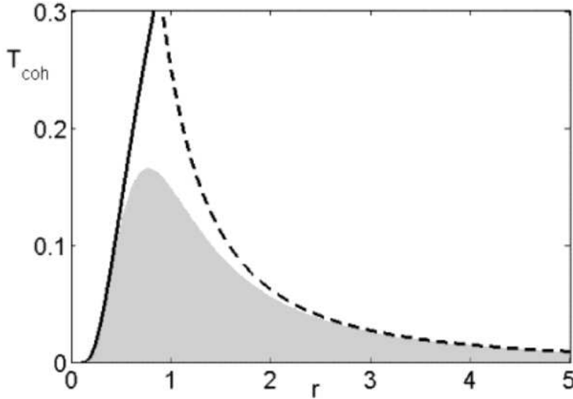
Figure 4. Estimates of the coherence temperatures in Ryd. for the BCS limit (solid line, Eq. (31)) and the BEC limit (dashed line, Eq. (32)). The parameter A = 1 and the scale for the BCS limit has been fit to the calculations of coupled quantum wells of [40], and m_e = m_h . The gray hatching is a smooth interpolation between the limits.
