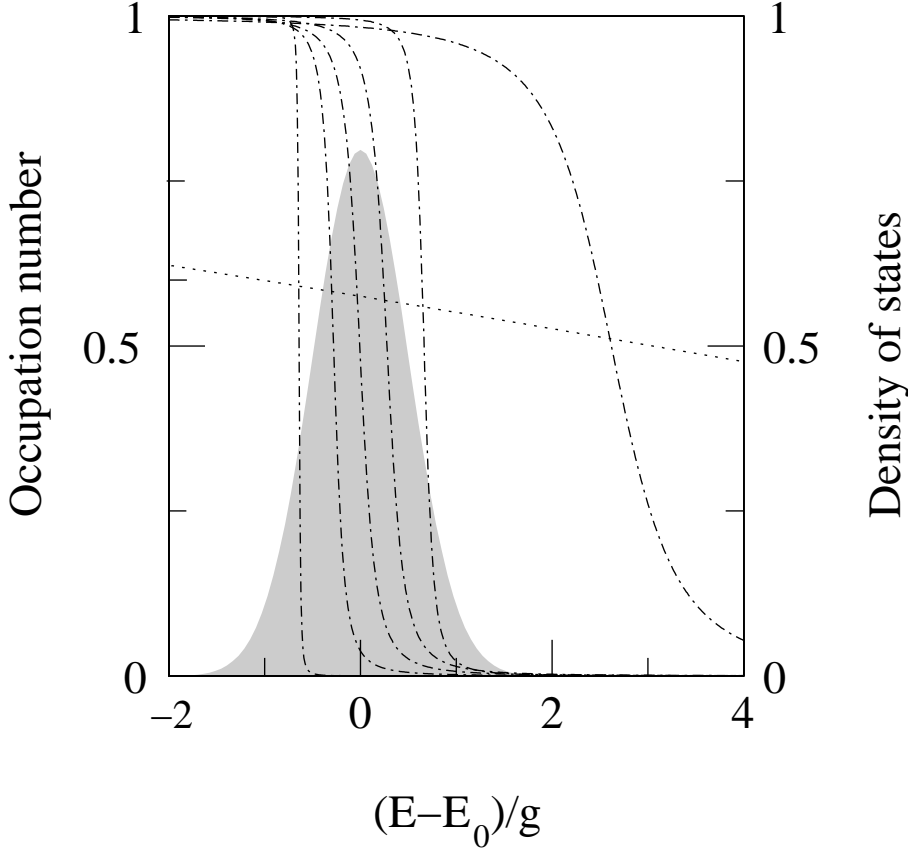
Figure 5. Occupancy v(\epsilon) as a function of two level system energy \epsilon where the photon energy is substantially detuned (above) the centroid of the exciton distribution ( \omega_c - \langle \epsilon \rangle = 3g ). The different curves correspond to \rho_x = 0.1, 0.3, 0.5, 0.7, 0.9 (dot-dash increasing from left to right) and \rho_x = 101 (dotted curve). The grey hatching is the density of states \nu(\epsilon) of the two-level systems. From [27].
