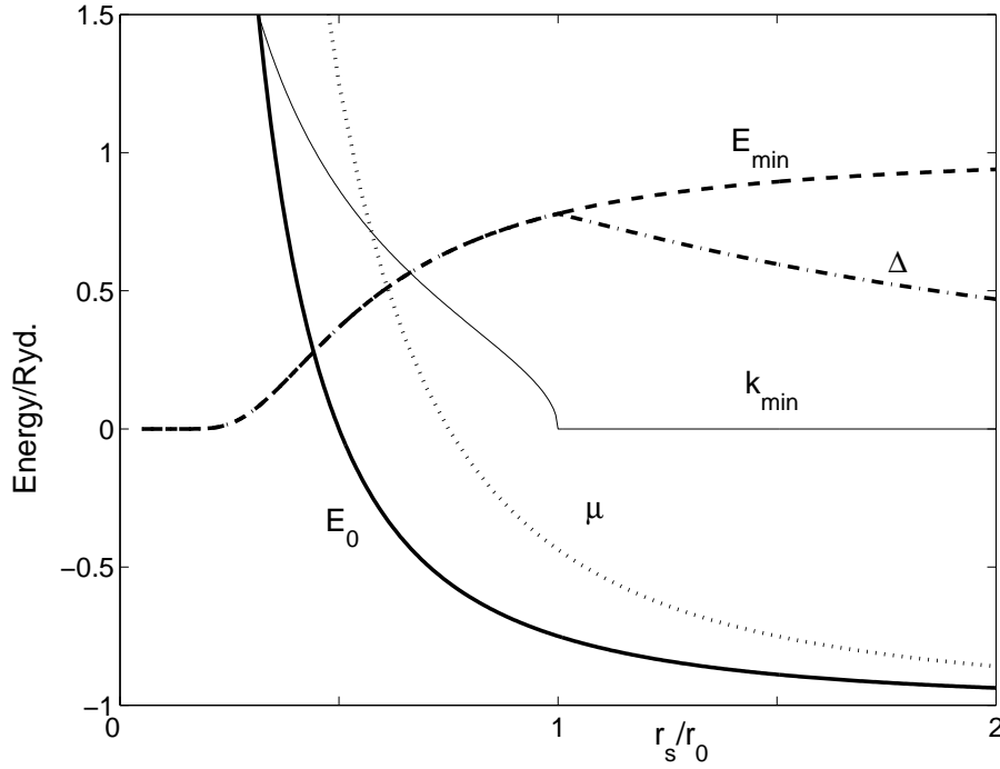
Figure 2. Sketch of the energy per particle E_0 (solid line) and chemical potential \mu (dotted) relative to the band edge, along with the correlation gap \Delta = \Delta(k_{min}) (dash-dot). Also shown is the minimum excitation energy E_{min} = \min(E_k) (dashed) and the wavevector k_{min} (thin solid line) of the minimum gap. Typically, the density parameter r_0 marking the BCS-BEC crossover is around 2-3.
