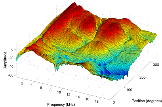
Figure 12: Reconstructed HRTFs. Length f = 430
