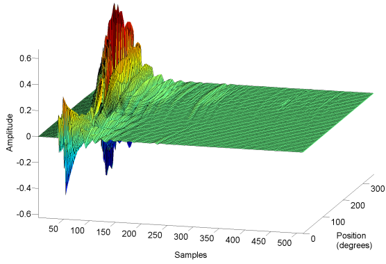
Figure 10: Reconstructed HRIRs. Length f = 430
