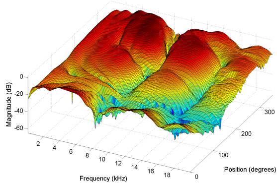
Figure 13: g^\phi components in frequency domain. Length f = 430
