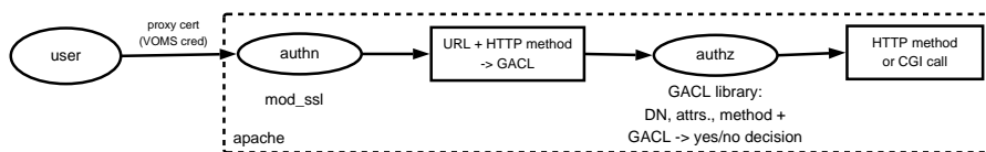
Figure 4. Authentication and Authorization in Apache
