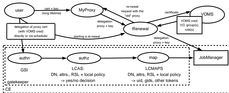
Figure 2. Authentication and Authorization in a Computing Element
