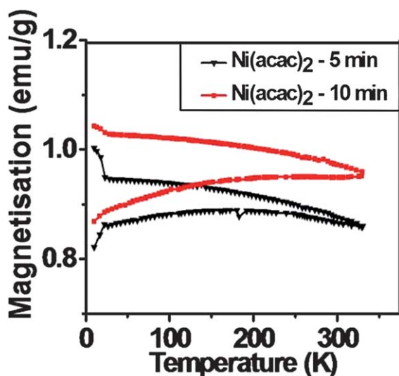
Fig. 9 Field-Cooled (FC) and Zero-Field-Cooled (ZFC) measurements taken with 10 Oe of magnetic field strength applied. The lower portion of each of the curves represents the ZFC measurement and the upper portion represents the FC measurement.
