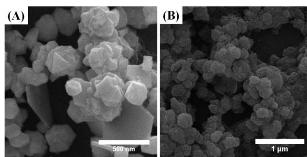
Fig. 5 SEM images of nickel particles synthesised using nickel acetylacetonate as the metal precursor, with a hold time of 10 minutes; using (a) 3 \times 10^{-4} mol and (b) 9 \times 10^{-4} mol of sodium formate.
