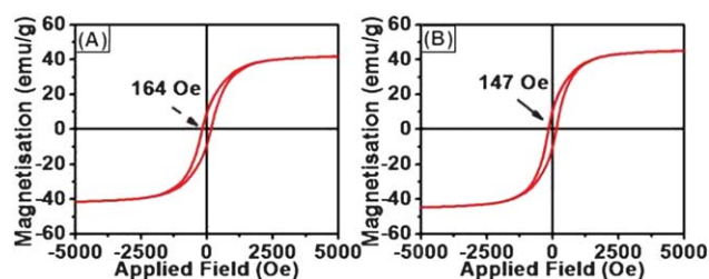
Fig. 6 Room temperature (300 K) hysteresis loops for samples prepared with the nickel acetylacetonate precursor with a microwave hold time of (a) 5 min and (b) 10 min. Coercivity values for the samples are shown in the graphs.
