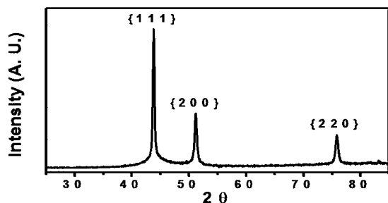
Fig. 4 X-Ray diffractogram of nickel nanocrystals prepared using nickel acetylacetonate as the metal precursor, with a microwave hold time of 10 min.
