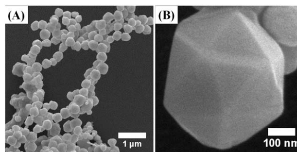
Fig. 2 (a) SEM images of nickel nanocrystals prepared using nickel acetylacetonate as the metal precursor with a microwave hold time of 10 minutes. (b) High magnification SEM image of the nickel nanocrystals shown in (a).
