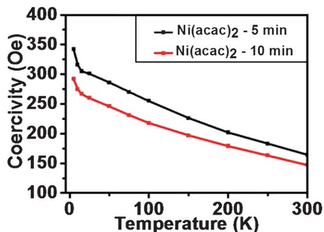
Fig. 8 Measurement of sample coercivity versus temperature for nanocrystal samples prepared using nickel acetylacetonate with varying hold times.
