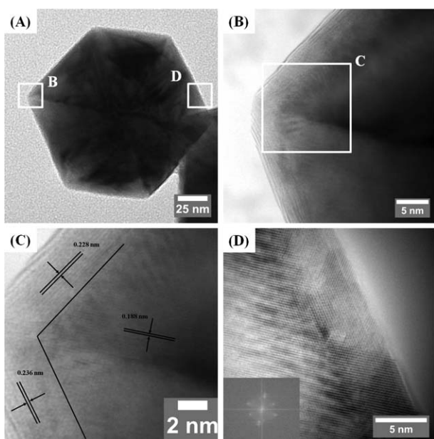
Fig. 3 TEM images of a single, icosahedral nickel nanocrystal, synthesised using nickel acetylacetonate as the metal precursor with a microwave hold time of 10 minutes. The outlines in (a) represent the areas shown in (b) and (d) while the outline in (b) represents the area shown in (c). The Fast Fourier Transformation (FTT) pattern of the nickel nanocrystal is shown in the inset of (d).
