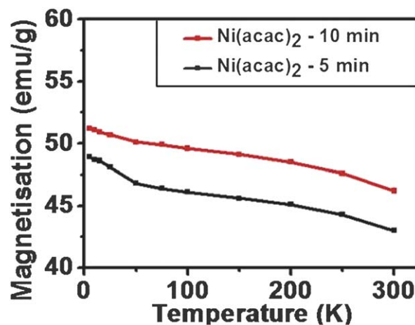
Fig. 7 Magnetisation versus temperature for nanocrystal samples prepared using nickel acetylacetonate with varying hold times.
