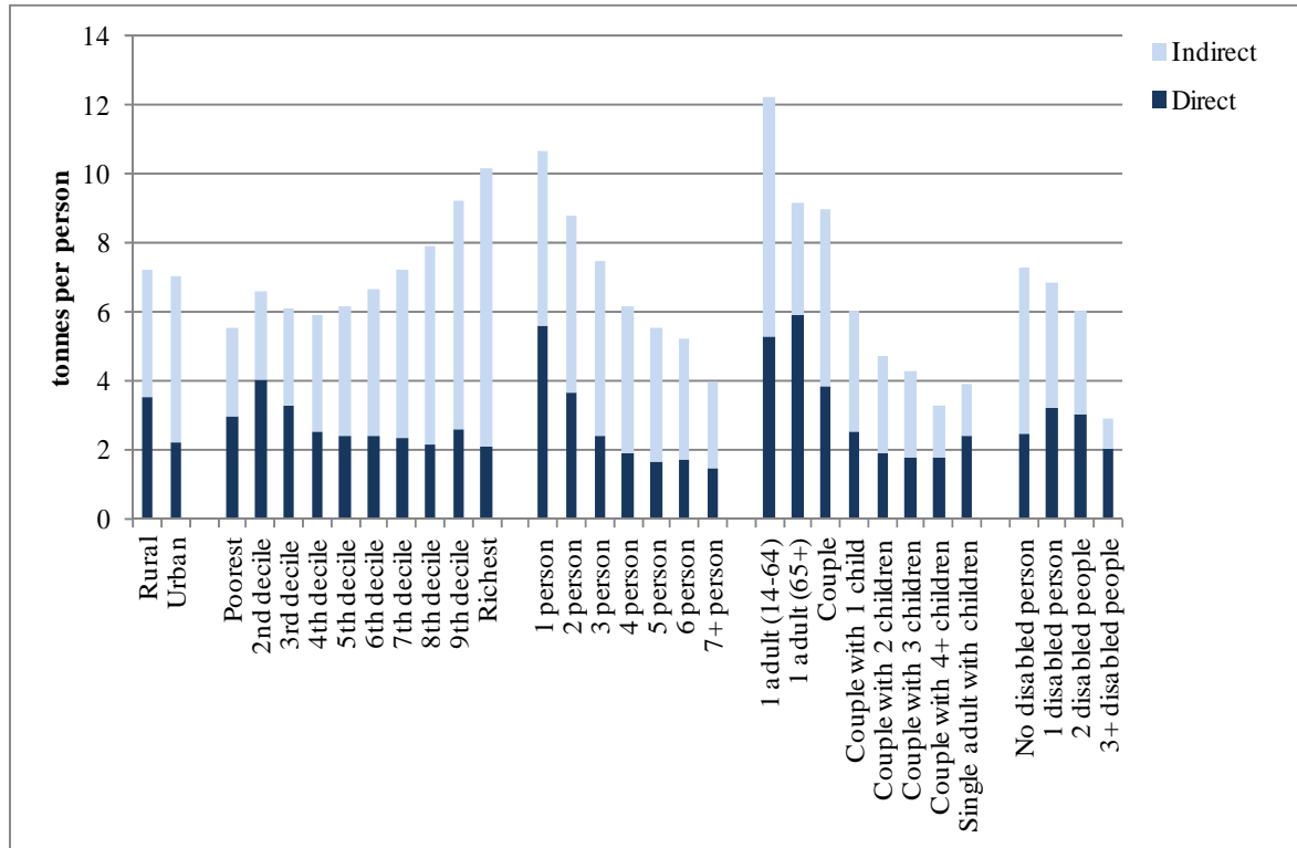
Figure 6: Direct and Indirect Emissions of Sulphur Dioxide per person by household type
