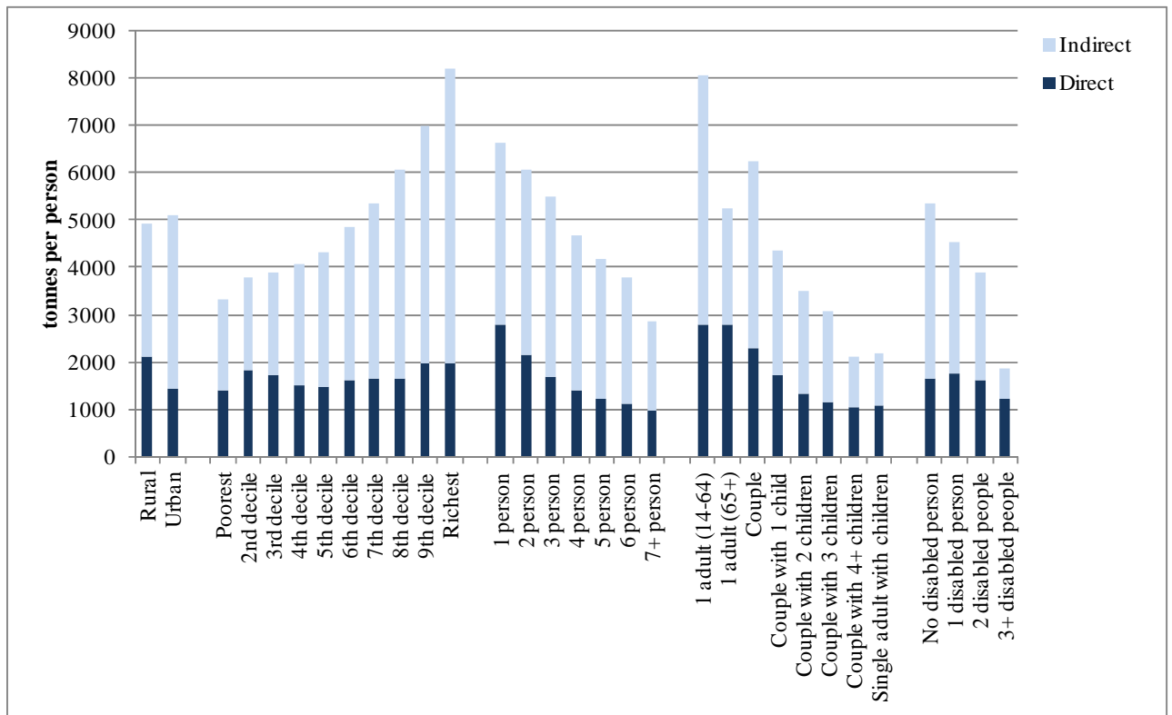
Figure 3: Direct and Indirect Emissions of Carbon Dioxide per person by household type
