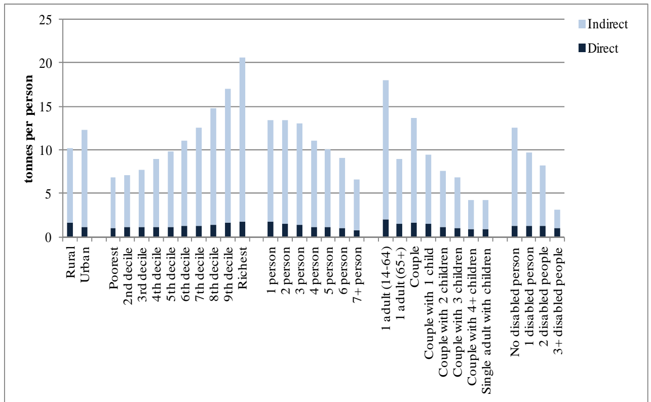
Figure A5: Direct and Indirect Emissions of Nitrogen Oxide per person
