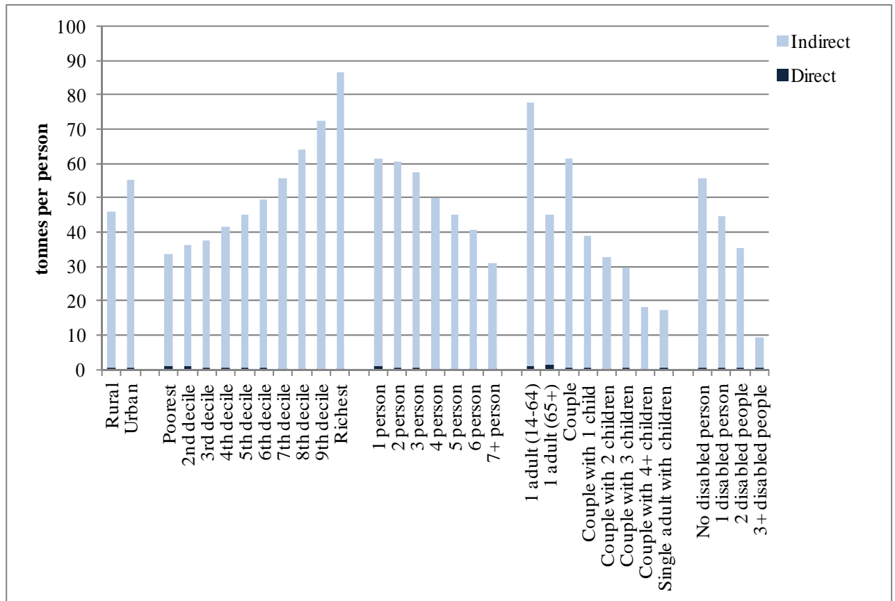
Figure 4: Direct and Indirect Emissions of Methane per person by household type
