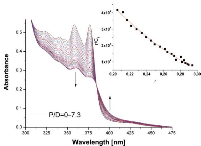
Fig. 5 UV/vis absorption spectra of rac -[Cr(phen) 2 (F 2 dppz)](CF 3 SO 3 ) 3 ( rac-3 ), (24 \mu M in 100 mM phosphate buffer solution, pH=7.4) in the presence of increasing concentrations of CT-DNA (P:D = nucleotide:Cr = 0–7.3). Inset: The Scatchard plot for rac-3 calculated using the absorbance at 377 nm ( r is the average number of bound complexes per base pair, C_1 is the concentration of the unbound complexes). The data were fitted between 20% and 90% bound complexes using the McGhee and von Hippel model. Nonlinear least squares regressions were done in ‘Origin 7.5’ based on the Levenberg-Marquardt algorithm.
