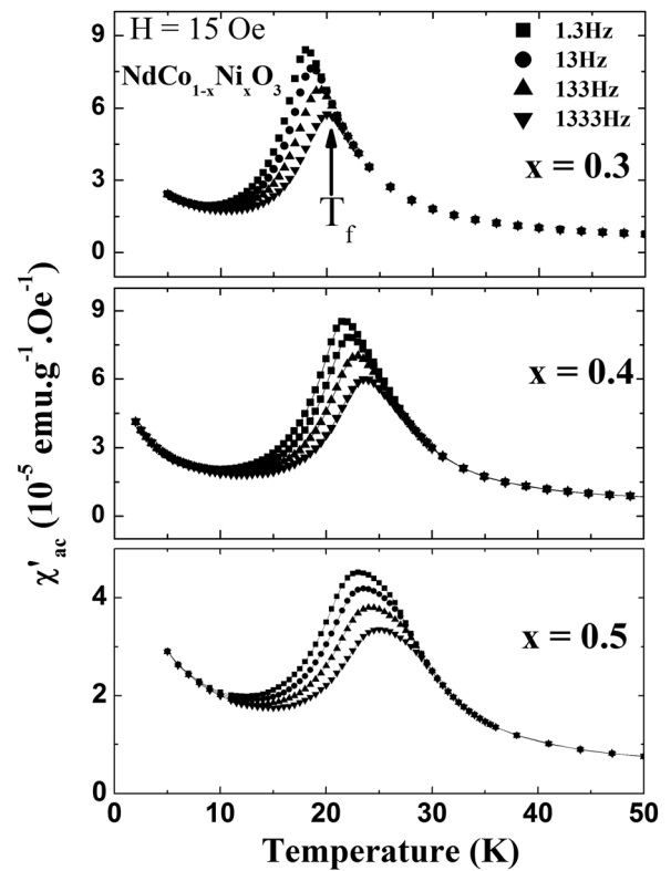
FIG. 5. The variation of AC magnetic susceptibility with temperature at different frequencies for x \geq 0.3 . T_f represents the spin glass freezing temperature. The shifting of peak position to higher temperature with increase in frequency is clearly seen.
