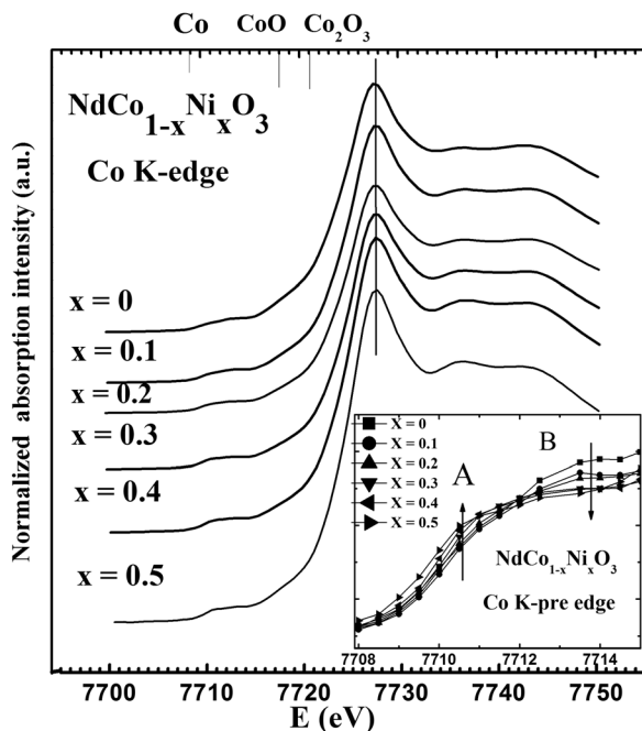
FIG. 2. XANES spectra for Co K-edge of \text{NdCo}_{1-x}\text{Ni}_x\text{O}_3 ( 0 \leq x \leq 0.5 ). No edge shift is observed on substitution. The enlarged view of pre edge region is shown in inset. The arrows indicate the shift in the spectral response with substitution.
