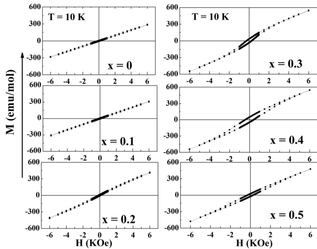
FIG. 6. Isothermal Magnetization hysteresis loops ( M - H ) of \text{NdCo}_{1-x}\text{Ni}_x\text{O}_3 ( 0 \leq x \leq 0.5 ) at 10 K. Change in the shape of the plots with substitution indicates to the coexistence of AFM and FM ordering for samples with x \geq 0.3 .
