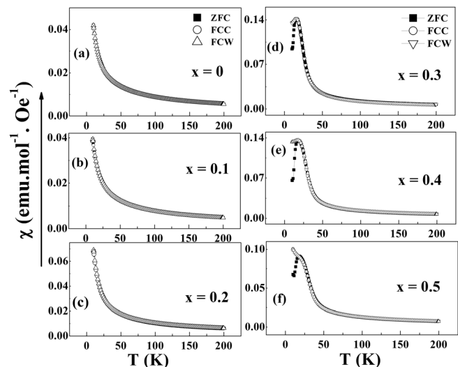
FIG. 4. Temperature dependence of dc magnetic susceptibility under different modes at a field of 1 kOe for \text{NdCo}_{1-x}\text{Ni}_x\text{O}_3 ( 0 \leq x \leq 0.5 ). Solid squares represent ZFC, open circles show FCC and open triangles are for FCW mode. A bifurcation in ZFC and FC curves appears after x=0.2 , which shows a composition dependent magnetic behaviour at low temperature.
