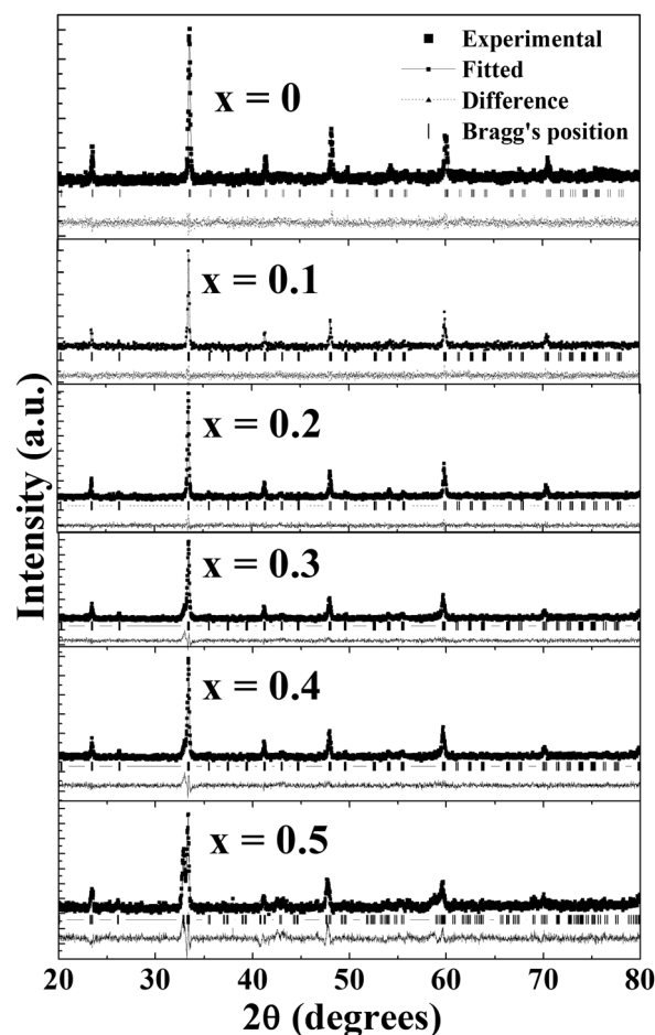
FIG. 1. Reitveld refined X-ray diffraction patterns for the samples NdCo 1-x Ni x O 3 ( 0 \leq x \leq 0.5 ). In each panel, solid squares represent observed data, and the line shows the calculated profile. The difference between the observed and the calculated pattern is shown at the bottom.
