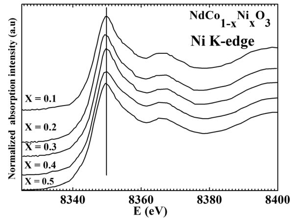
FIG. 3. XANES spectra for Ni K-edge of \text{NdCo}_{1-x}\text{Ni}_x\text{O}_3 ( 0.1 \leq x \leq 0.5 ). Clear indication of +3 valence state of Ni appears in all composition.
