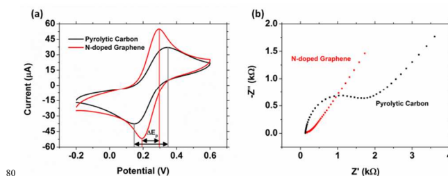
Fig. 4 (a) Cyclic voltammograms of as-grown PyC (black) and N-doped graphene on PyC (red), peak separation ( \Delta E_p ) is marked. The scan rate is 100\text{ mV s}^{-1} (b) Corresponding Nyquist plots for the two materials.
