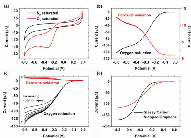
Fig. 5 (a) Cyclic voltammograms for N-doped graphene in \text{N}_2 saturated (black) and \text{O}_2 saturated (red) 1 M NaOH. (b) LSVs for RDE measurement of N-doped graphene showing currents owing to oxygen reduction (black) and peroxide oxidation (red); rotation speed of 2000 rpm. (c) A series of LSVs for the same material at various rotation speeds, ORR and peroxide currents are included. (d) LSVs for RDE measurements of GC (black) and N-doped graphene (red).
