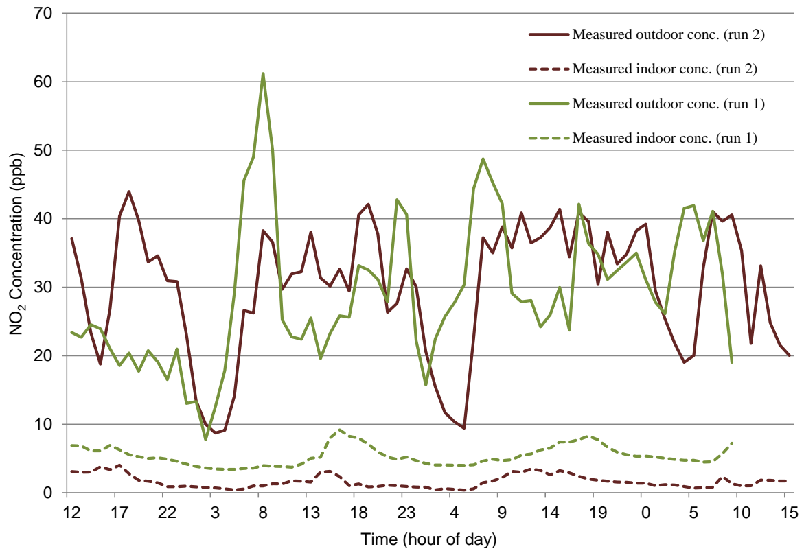
Figure 7. Measured indoor and outdoor NO 2 concentrations at N t 2 (run 1 and run 2).
