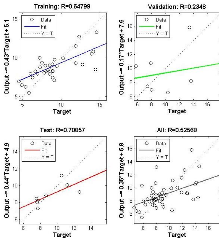
Figure 4. M_c2 run 1 PM_{2.5} regression of trained output data set.
