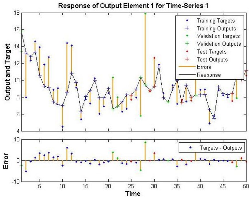
Figure 3. Time series of neural network training M_c2 run 1 PM_{2.5} .
