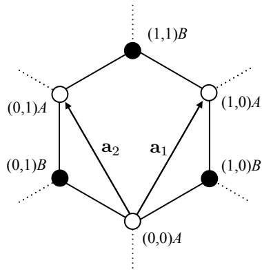
FIG. 3. Schematic representation of the lattice labels i = (m, n) corresponding to \mathbf{R}_i = m\mathbf{a}_1 + n\mathbf{a}_2 . For the top-bonded case, the impurity is placed atop of the (0,0) site, whereas for the center-bonded case, the impurity is at the center of the hexagonal ring.
