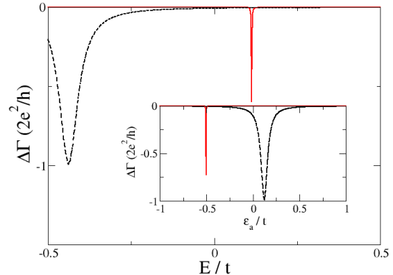
FIG. 4. (Color online) Change in the conductance \Delta\Gamma (in units of 2e^2/h ) as a function of the Fermi energy for a single impurity with on-site energy \epsilon_a = -0.5t , and \tau = -0.5t . Solid red (dashed black) line corresponds to the case of a centre-bonded (top-bonded) impurity. Inset depicts the same quantity for a fixed Fermi energy E_F = 0.11t , this time plotted as a function of the impurity's on-site energy.
