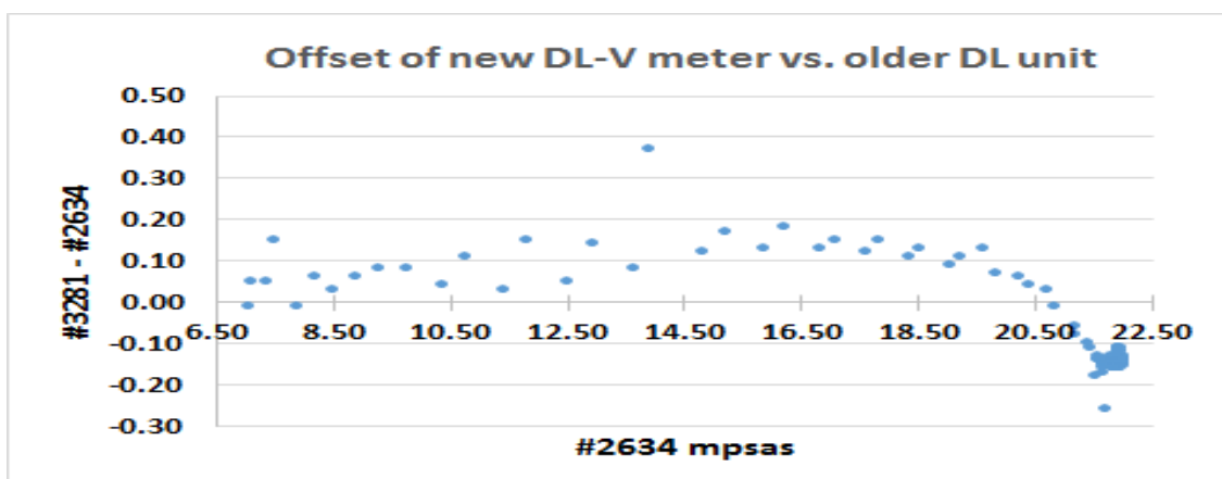
Figure 36: A plot of the differences of the new vector SQM unit relative to the older data-logging unit taken in evening twilight on 2 May. Note that the agreement is generally good, with deviations becoming apparent for magnitudes fainter than 19.5 - compare this plot with Figure 40 below.
