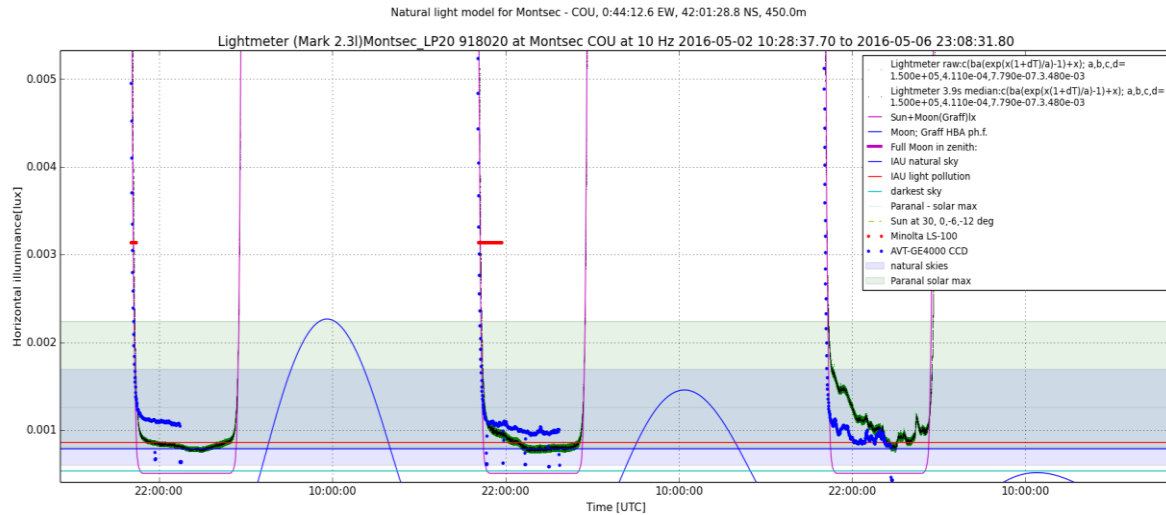
Figure 31: Horizontal illuminance measured by the Lightmeter (black) and 1^\circ aperture zenithal luminance by the AVT-CCD (blue) and the Minolta LS-100 (red) converted to illuminance assuming isotropy of the sky hemisphere. mLux-region with linear ordinate. The dashed horizontal line marks the light levels of a clear sky at the end of nautical twilight, shades are Paranal natural skies. Luminance measurements by Costas Bouroussis
