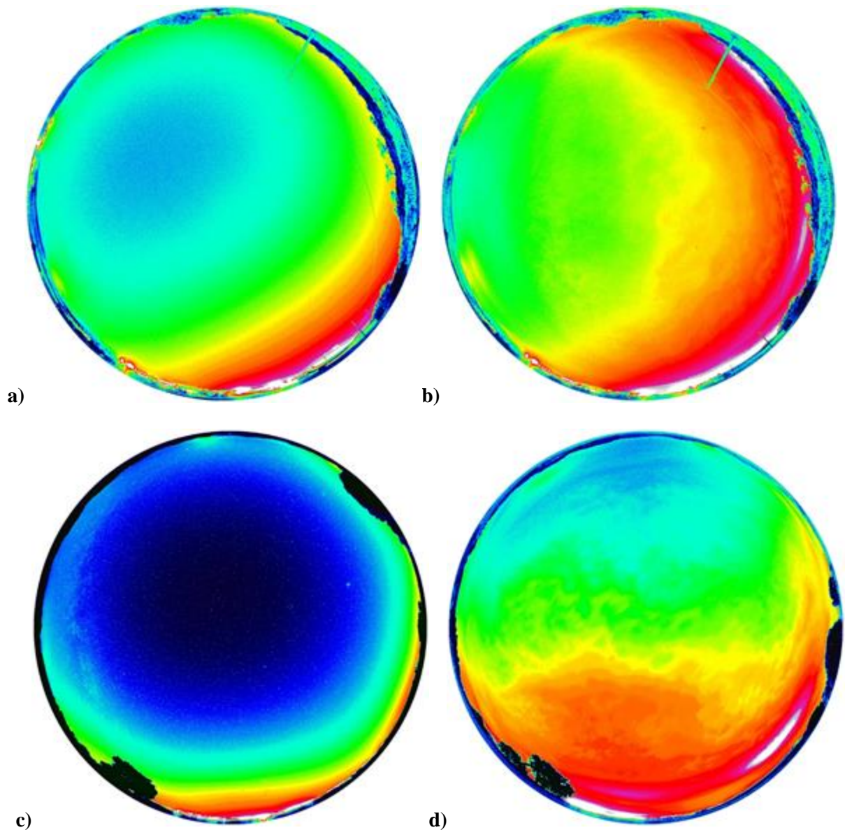
Figure 12: False color luminance plots from all-sky pictures taken at two stops of the transect form Balaguer to Port d'Àger: a) Location LONNE3 clear conditions b) Location LONNE3 partly cloudy conditions; c) d)
