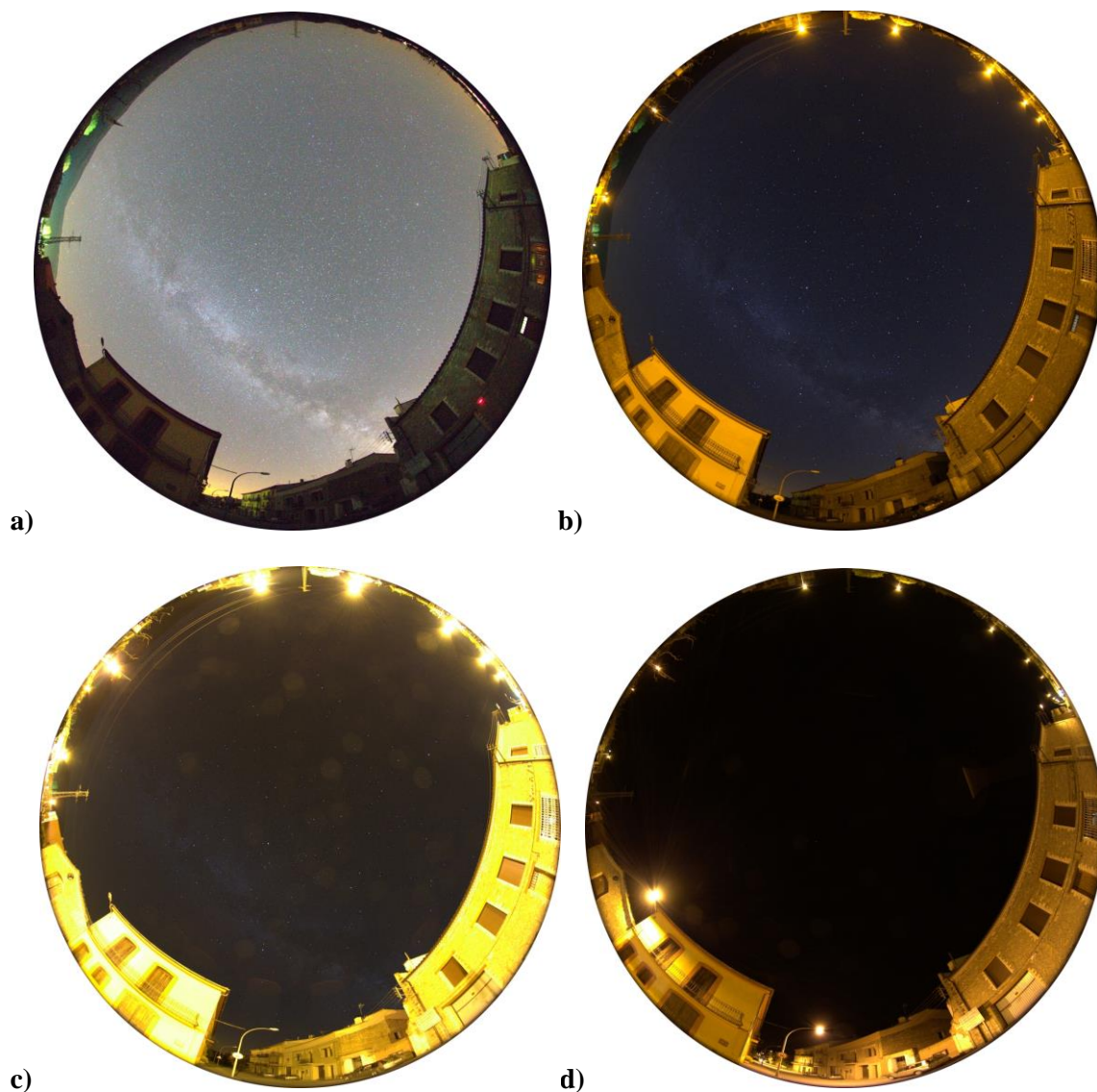
Figure 13: All-sky pictures taken in Àger during the switch-on of the lights on May 4th 2016 a) 4:21 am; b) 4:23 am; c) 4:27 am; d) 4:35 am.
