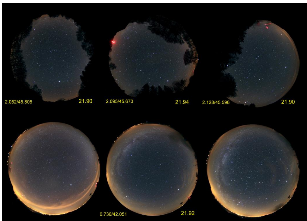
Figure 4: Top: all-sky pictures (Canon D550, 2.8/4.5mm, ISO 800, 3 min) from PNR de Millevache en Limousin (3 places with long/lat and SQM brightness ), Bottom: same next night from Parc Astronòmic Montsec-COU.
