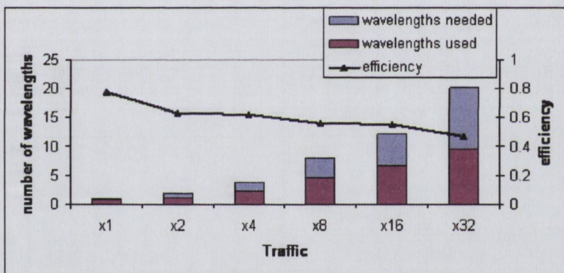
Figure 4.4: Wavelength efficiency using the first fit algorithm
