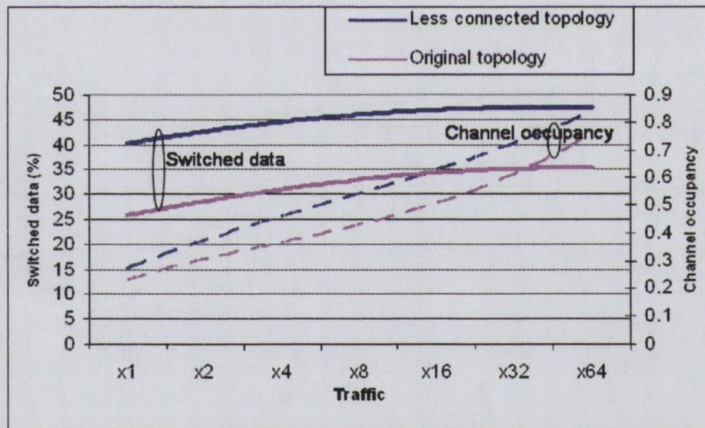
Figure 4.9: Network performance with reduced average node degree
