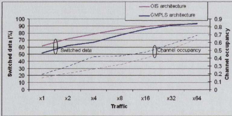
Figure 4.15: OIS vs. GMPLS architecture for interdomain switching
