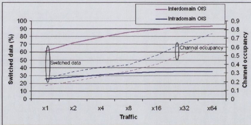
Figure 4.13: Interdomain vs. intradomain OIS performance in GÉANT
