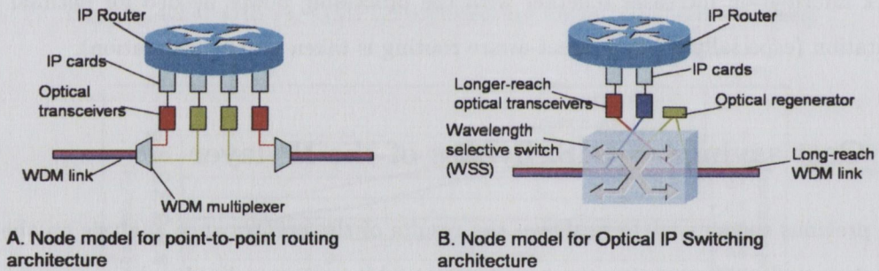
Figure 4.16: Node models for the cost analysis
