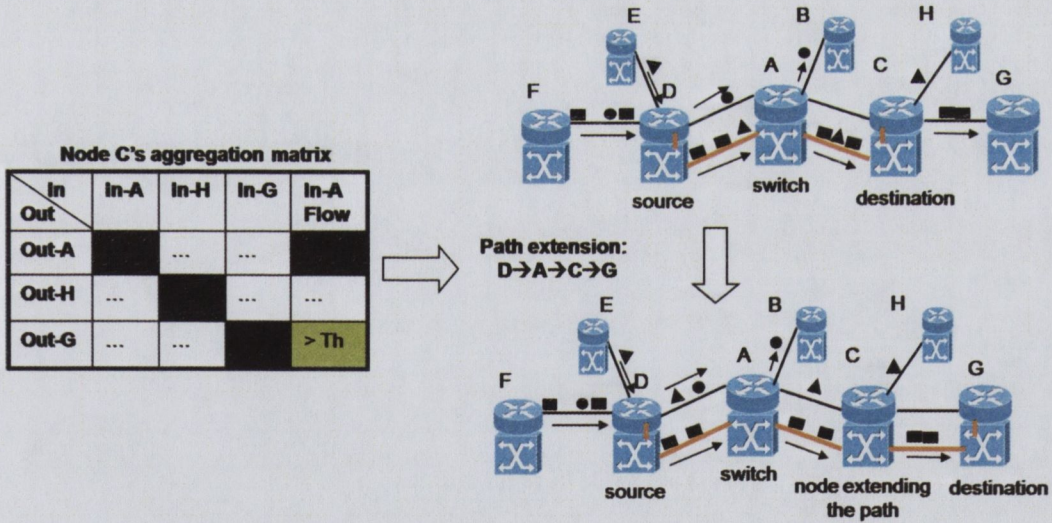
Figure 3.10: Path extension process
