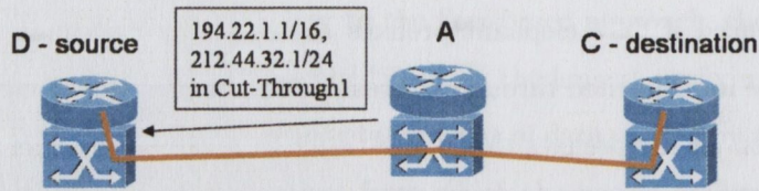
Figure 3.7: Signaling of switched prefixes
