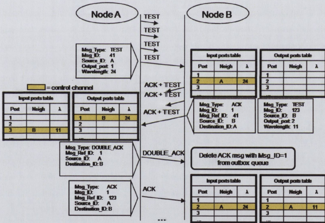
Figure 3.28: Example of messages exchanged by the link discovery protocol
