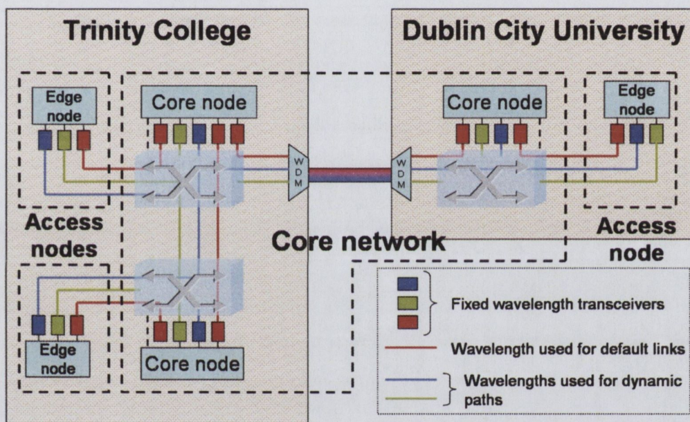
Figure 5.1: Network architecture of the OIS testbed
