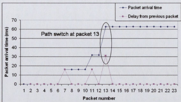
Figure 5.8: Path creation test results for burst interval times of 15 ms
