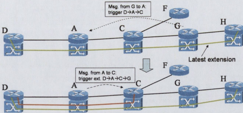
Figure 3.13: Example of path restoration
