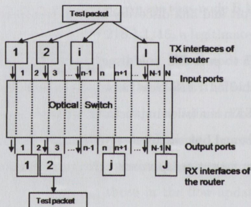
Figure 3.20: First iteration of the parallel algorithm
