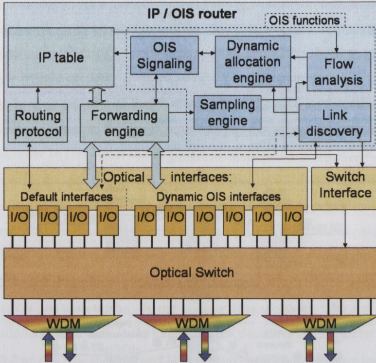
Figure 3.2: Overall Optical IP Switching architecture
