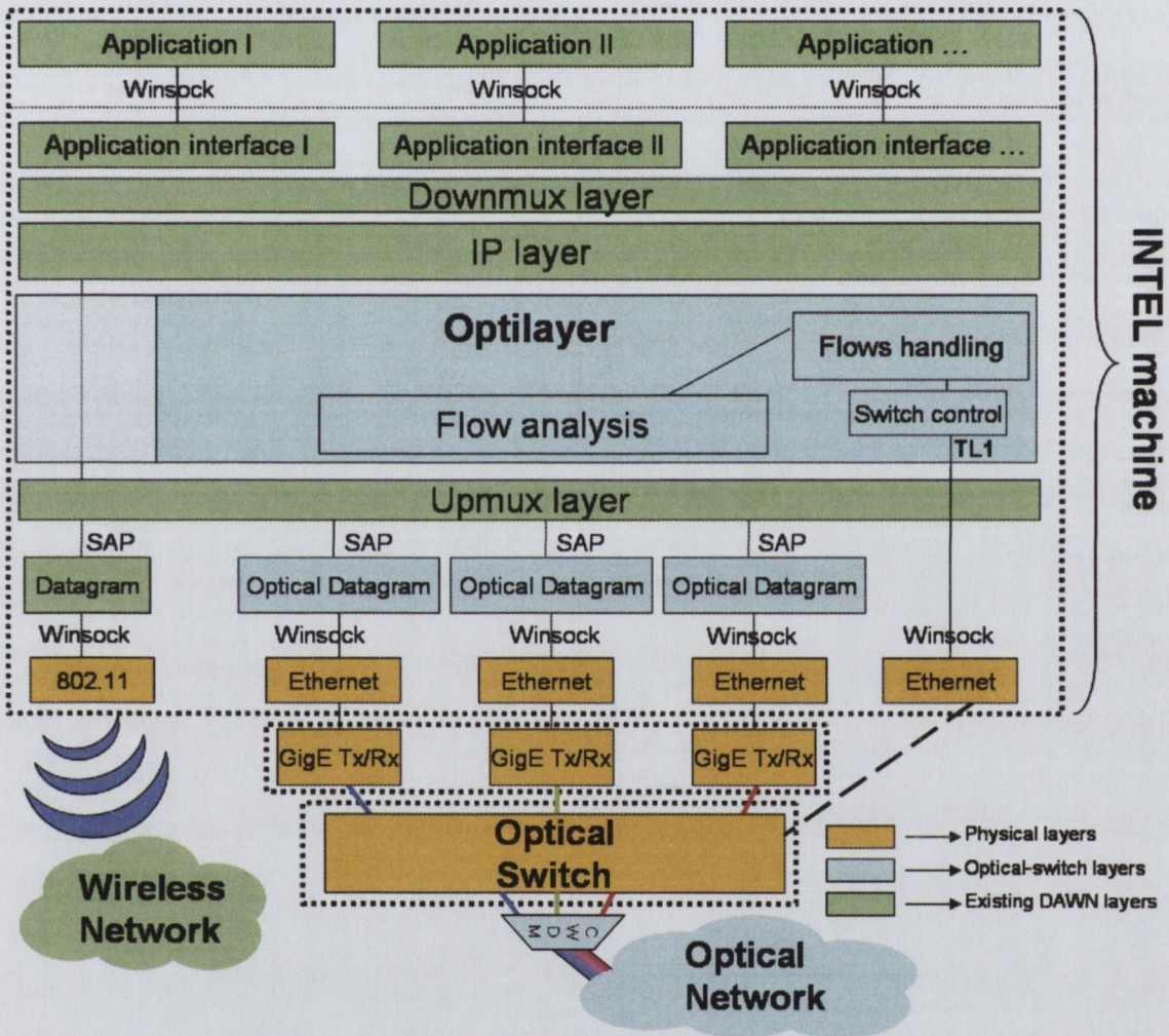
Figure 5.2: OIS testbed node architecture
