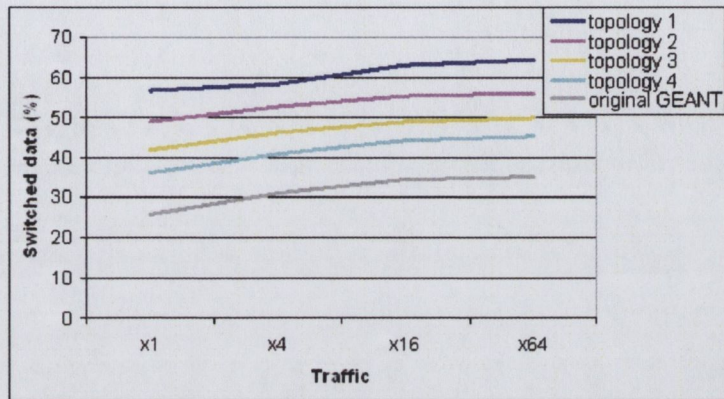
Figure 4.11: Simulation results using different network topologies
