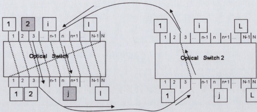
Figure 3.27: Example of configuration that could confuse the discovery process
