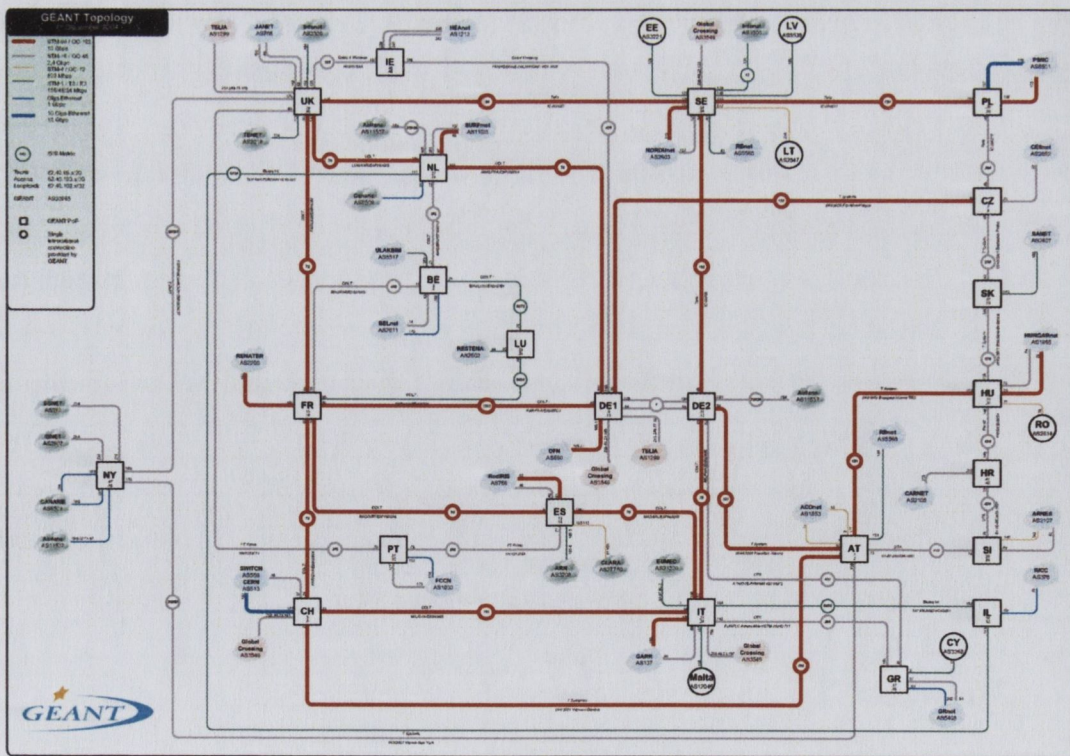
Figure 4.1: GÉANT logical layout topology
