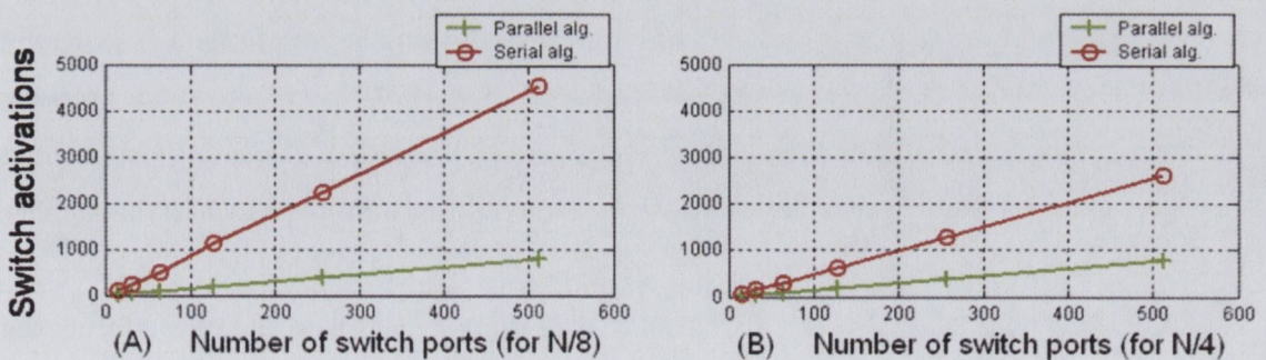
Figure 5.4: Average number of switch activations required to complete the discovery process
