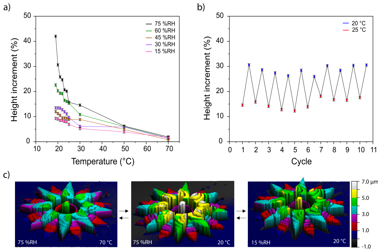
Figure 4. Characterization of the actuation of a flower at different atmospheric conditions and temperatures. a) Height changes of the flower over a ranges of different temperature and humidity values. b) Increment of the flower height over ten cycles, going from 25 °C to 20 °C, at 75 ± 2 %RH. For both a) and b), the percentage of height increment is obtained by averaging the values of the top of the flower and comparing them to the height of the flower before base treatment. For all measurements, the flower was held for 5 min after reaching the desired conditions before recording its height. Error bars represent standard deviations for N=3 measurements. c) 3D profiles of the flower which depict direct (triggered by humidity) or indirect (triggered by temperature) actuation.
