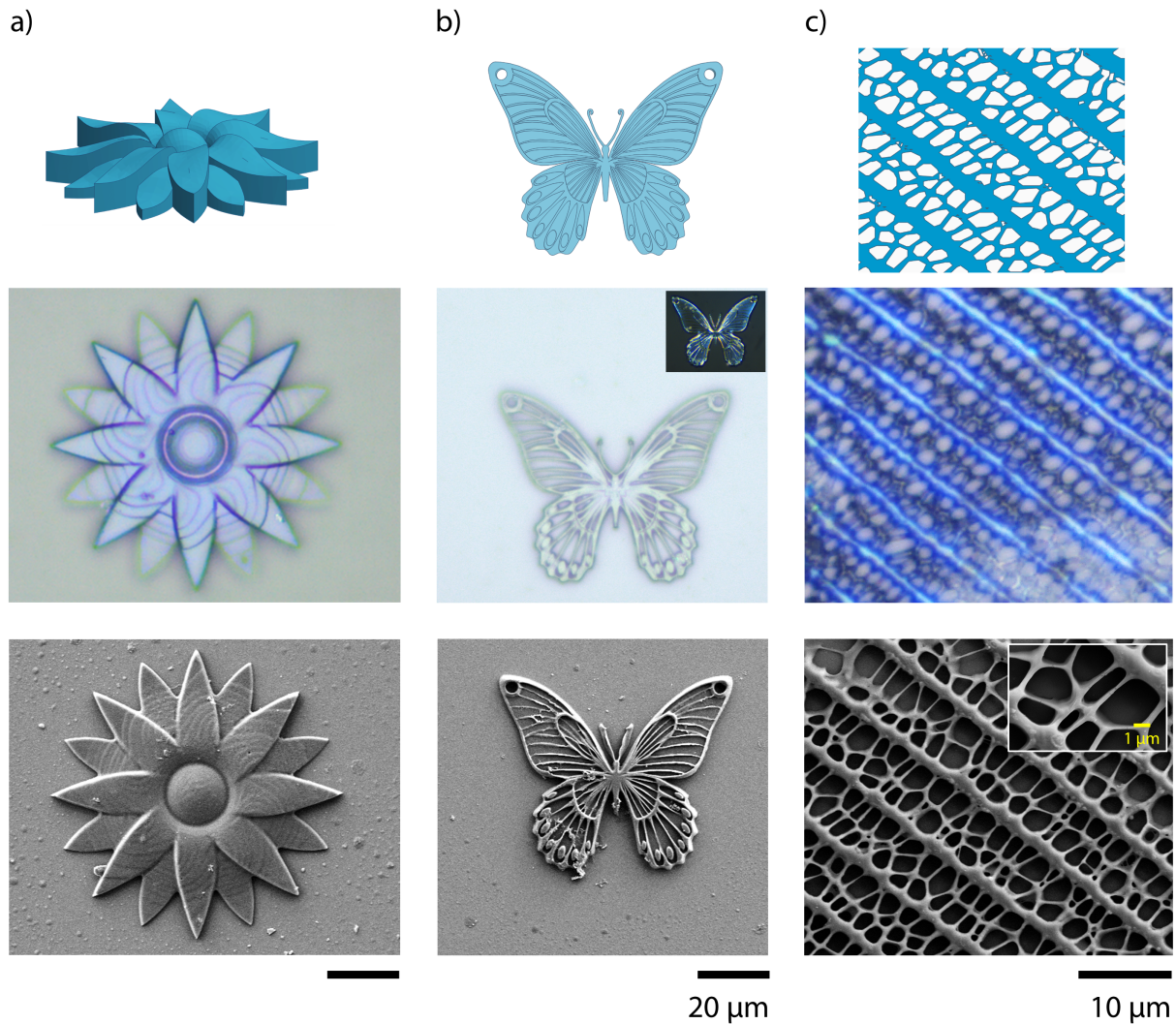
Figure 3. Photonic 3D microstructures. From top to bottom, the CAD designs of the structures, optical microscopy and SEM images before base treatment of (a) a flower, (b) a butterfly, and (c) the pattern of the wing of the Papilio paris butterfly. The inset in b) is a crossed linear polarized micrograph of the butterfly, used to enhance observation of the reflected color.
