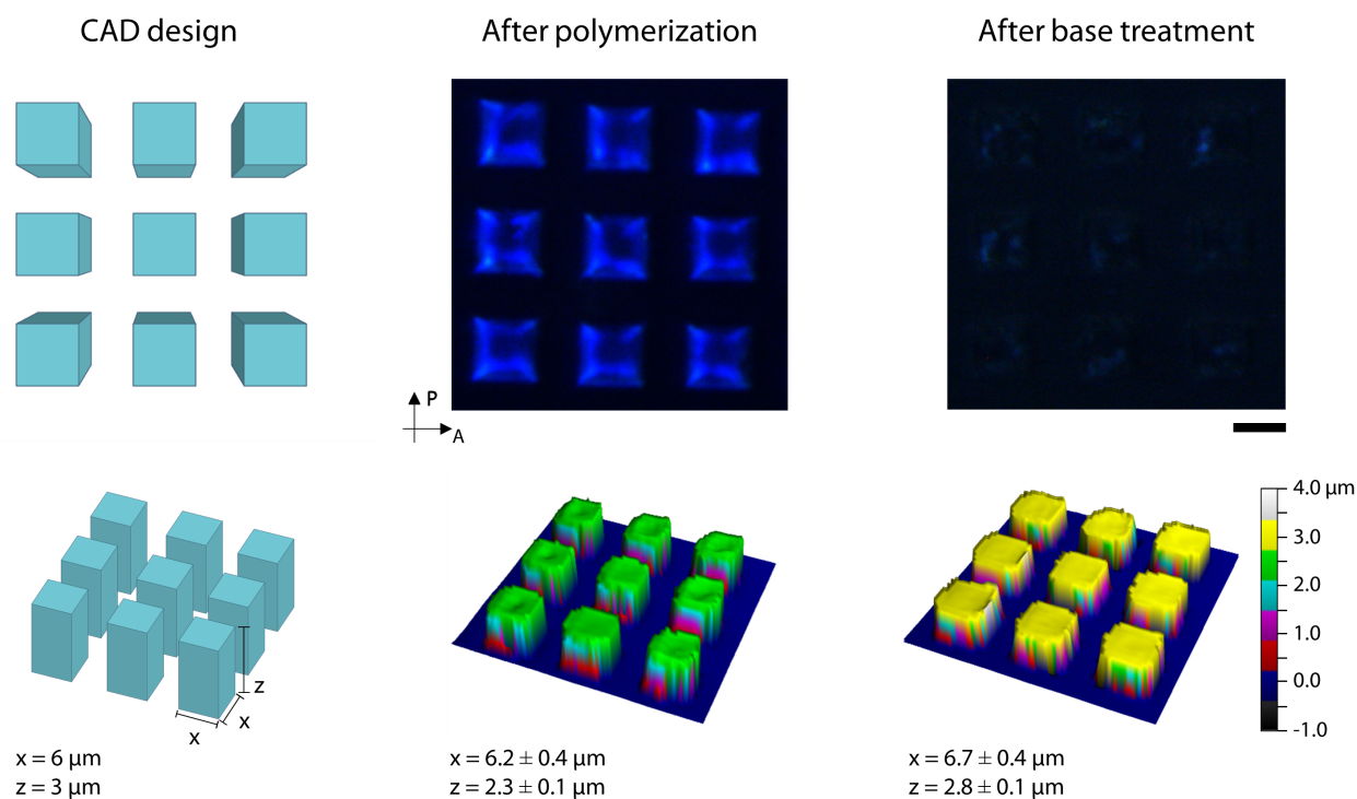
Figure 2. Structural and optical characterization of an array of pillars after polymerization and after base treatment. Top-crossed polarized micrographs; bottom-3D profiles of the array of pillars. The scale bar represents 10 \mu\text{m} .
