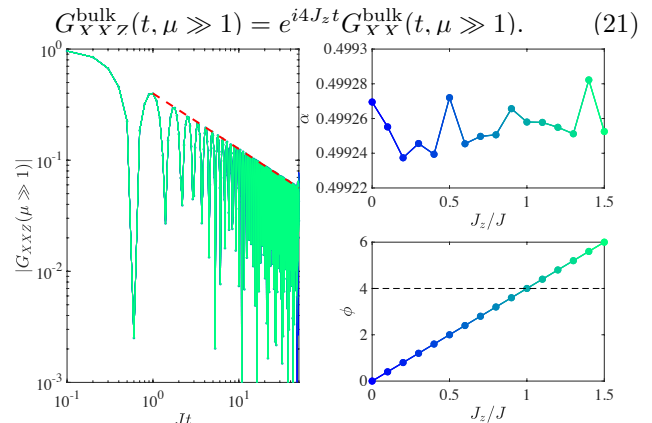
FIG. 6. MPS results for correlations with a chain of 200 spins in agreement with the analytical results. Darker colors correspond to lower J_z while brighter colors correspond to higher J_z . The modulus of the correlation in log-log scale for (Upper left) \mu \gg 1 . The red dashed line is the asymptotic expression in (19), respectively. The Bessel function result is indistinguishable from the MPS results. (Upper right) The fitted power law exponent and (lower right) the corresponding phase frequency assuming G_{XXZ} \sim e^{i\phi t} t^{-\alpha} . Thus we have confirmation that \alpha = 1/2 and \phi = 4J_z .
