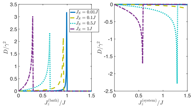
FIG. 4. Asymptotic Born results for the diode factor for (left) a non-interacting system with interacting leads and (right) an interacting-system with non-interacting leads. We set \Delta = J_S .
