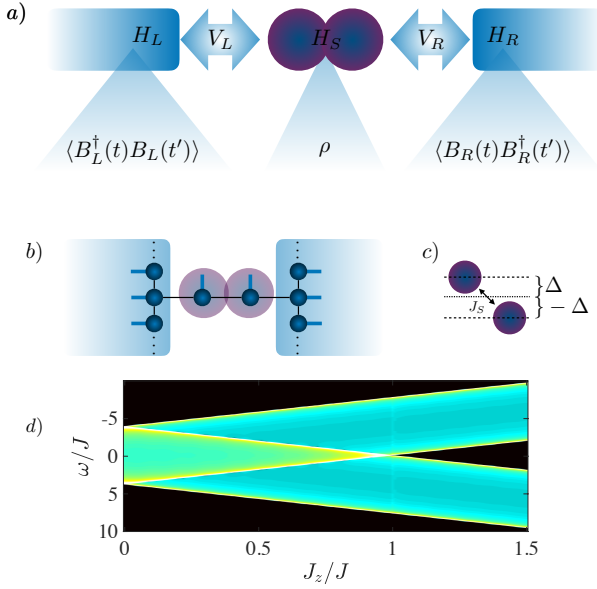
FIG. 1. a) Representation of bath-system-bath coupling and effective evolution of the central interface that depends on its past history and time correlations of the bath. b) The system-lead state |\Psi\rangle depicted as a matrix-product-state reflecting the corresponding Hamiltonian structure of bulk-coupling. c) The small asymmetric interface between the leads is represented as a two qubit structure. d) The system-bath asymptotic nonequilibrium spectral function A_{\Pi}(\omega) under the Born approximation for different J_z couplings showing the spectral structure of the bath with a gap around \omega = 0 for certain regimes in the limit H_S \ll H_B ( J_S, \gamma = 0.01J ).
