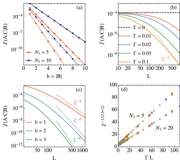
FIG. 5. Conditional mutual information (CMI) \mathcal{I}(A : C|B) [Eq. (4)] for a symmetric tripartition with the middle block having size b = |B| . (a) Log of the CMI as a function of b , for both the ballistic case ( \Gamma = 0 , solid lines) and diffusive case ( \Gamma = 0.1 , dashed lines), with different values of N_1 and fixed L = 40 and N_L = 1 . In both cases the CMI behaves as \mathcal{I}(A : C|B) \sim 1/R^b , where R > 1 is a constant that depends on the temperature gradient. (b) Log-log plot of the CMI as a function of L for b = 1 . If \Gamma = 0 then \mathcal{I}(A : C|B) is independent of L , whereas for \Gamma \neq 0 we get \mathcal{I}(A : C|B) \sim 1/L^4 . (c) Log-log plot of the CMI vs. L for different values of b with N_1 = 15 , N_L = 1 and \Gamma = 0.1 . For large L the CMI scales as \mathcal{I}(A : C|B) \sim 1/L^{2b+2} . (d) Finite size scaling, Eq. (23), for two different values of N_1 , with N_L = 1 and multiple values of \Gamma , L and b . In all curves we set \gamma = \lambda = 1 .
