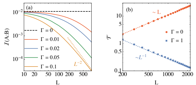
FIG. 4. (a) Log-log plot of the Mutual Information (MI) \mathcal{I}(A : B) [Eq. (1)] between two halves of the chain as a function of L , for different values of the self-consistent noise \Gamma . (b) Same but for the total correlations \mathcal{T} [Eq. (3)]. The curve for \Gamma = 1 was multiplied by 10^{-3} to improve visibility. In all curves we set N_1 = 2 , N_L = 1 and \gamma = \lambda = 1 .
