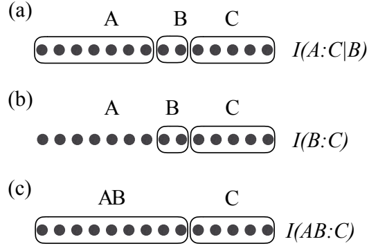
FIG. 2. The chain rule (5) connecting the MI (1) and the CMI (4).
