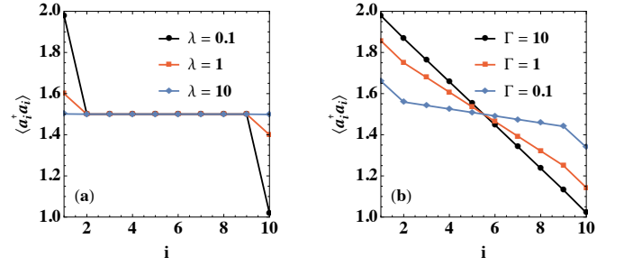
FIG. 3. Occupation profile \langle a_i^\dagger a_i \rangle as a function of the site number i . (a) Ballistic case ( \Gamma = 0 ) for different values of \lambda . (b) Diffusive case, with \lambda = 1 and different values of \Gamma . Other parameters are L = 10 , \gamma = 1 , N_1 = 2 and N_L = 1 .
