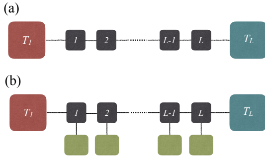
FIG. 1. (a) A boundary-driven one-dimensional quantum chain subject to two baths at each end. (b) By including additional noise sources within the chain, here implemented using the idea of self-consistent reservoirs, it is possible to tune the flow from ballistic to diffusive.
