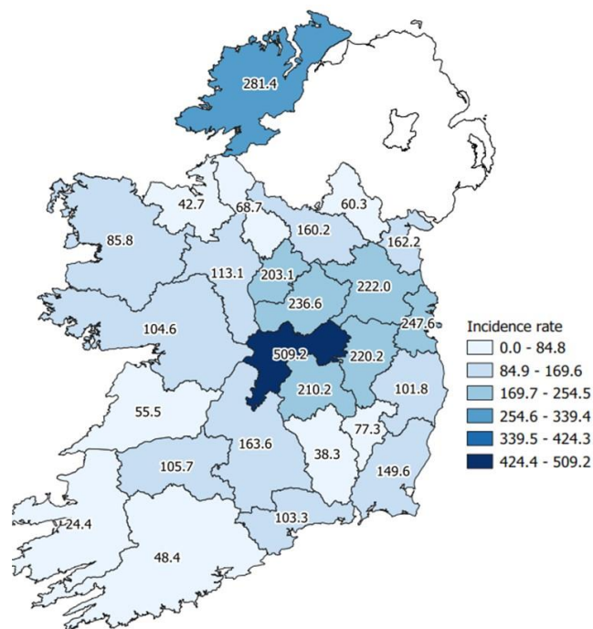
Cumulative 14-day incidence rates of confirmed cases of COVID-19 per 100,000 population notified in Ireland between 18/03/2021 and 31/03/2021
