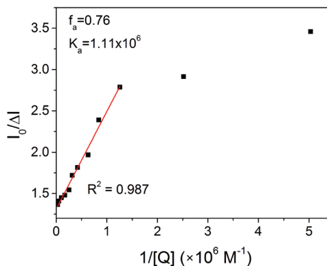
Fig. 3 Linear fit to buried fluorophore model of modified Stern–Volmer plot for fluorescence quenching of PF2/6- b -P3TMAHT by GTP ( \lambda_{ex} = 380 nm, \lambda_{em} = 480 nm).
