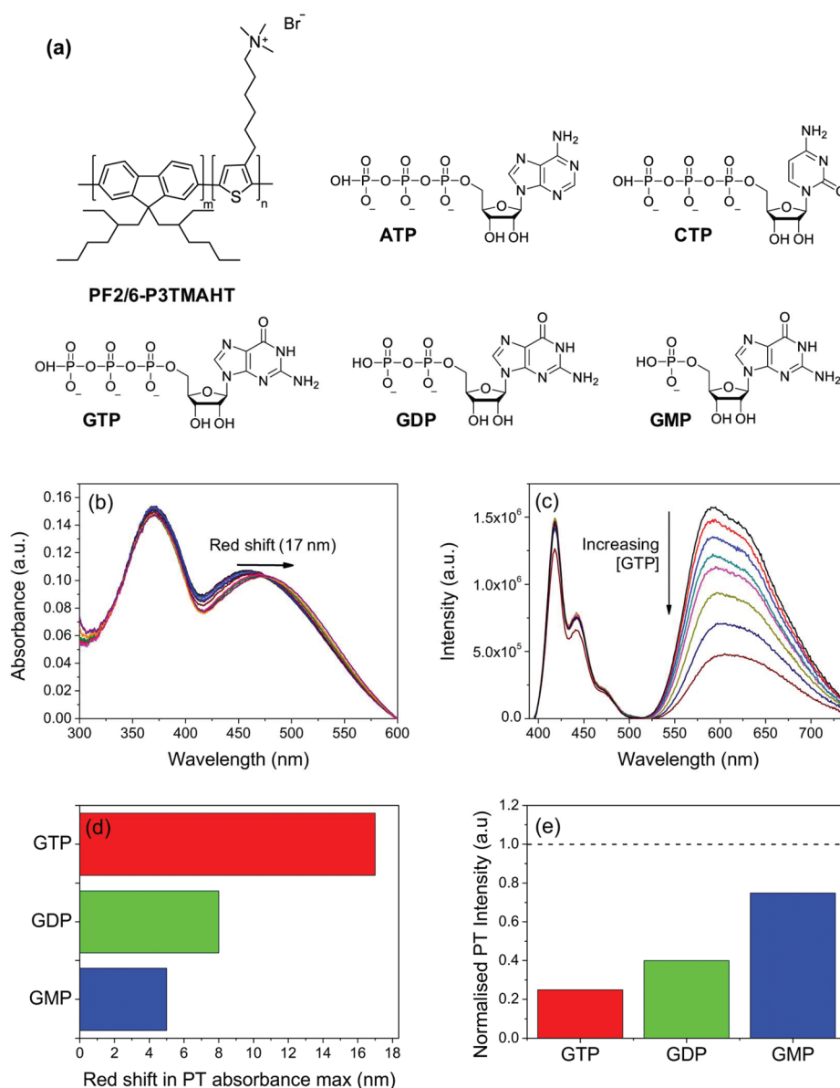
Fig. 1 (a) Chemical structures of the CPE ( PF2/6- b -P3TMAHT ) and the bioanions used: adenosine triphosphate (ATP); cytidine triphosphate (CTP); guanosine triphosphate (GTP); guanosine diphosphate (GDP) and guanosine monophosphate (GMP). (b) UV/Vis absorption and (c) PL spectra ( \lambda_{\text{ex}} = 380 nm) for PF2/6- b -P3TMAHT in aqueous solution in the presence of increasing concentration of GTP (0–38 \mu\text{M} ). (d) Magnitude of the red-shift in the PT absorption maximum and (e) intensity of the PT emission on addition of an excess of GTP, GDP and GMP, normalised relative to the initial PT emission intensity. The black dashed line serves only to guide the eye, indicating the relative intensity of the initial PT emission.
