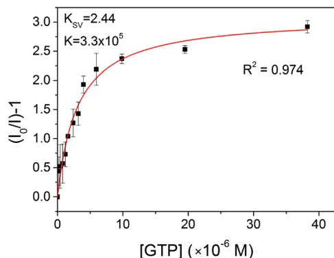
Fig. 4 Fit to a multi-equilibrium model of modified Stern–Volmer plot for fluorescence quenching of PF2/6- b -P3TMAHT by GTP ( \lambda_{\text{ex}} = 380 nm).
