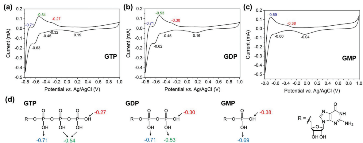
Fig. 5 Cyclic voltammograms for (a) GTP, (b) GDP and (c) GMP in H 2 O at 50 mV s -1 scan rate using Pt as the working and counter electrode, Ag/AgCl as reference electrode and KCl (0.1 M) as the supporting electrolyte. (d) Assignment of CV peaks for each reduction process depending on the number of phosphates present on the nucleotide.
