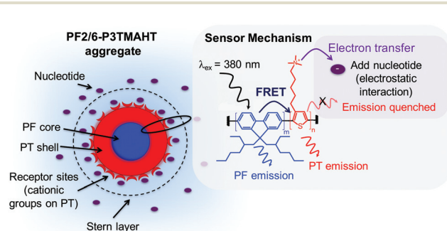
Scheme 1 Schematic representation of PF2/6- b -P3TMAHT ( m = 37 , n = 46 ) aggregates in water showing a PF rich core (blue) and PT shell (red) with the charged groups of the PT block acting as receptor sites on the aggregate surface. The sensor mechanism for the detection of nucleotides is also shown.
