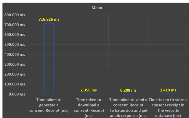
FIGURE 8. Integration of receipts with cookie banners.
