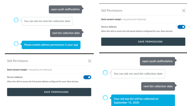
FIGURE 9. Implementing receipts in Alexa.
