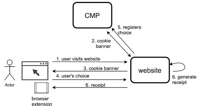
FIGURE 6. Integration of receipts with cookie banners.
